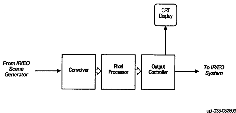
Figure 6 - UPI Top-level Architecture
