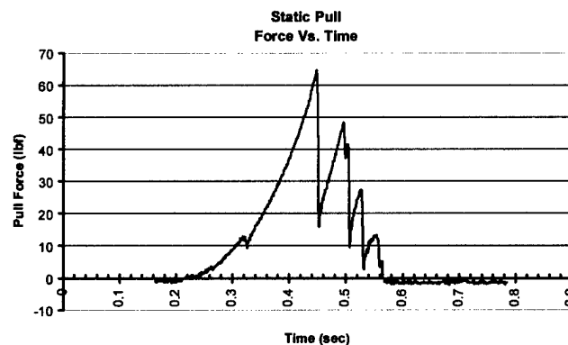
Figure 6 Typical Static Pull Test Force vs. Time
