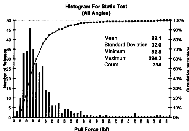
Figure 7 Static Test Histogram
