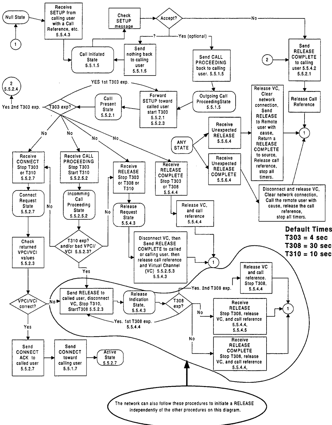
Figure 24. Control Plane – UNI 3.1 Call/Connection at Network ATM UNI Interface
