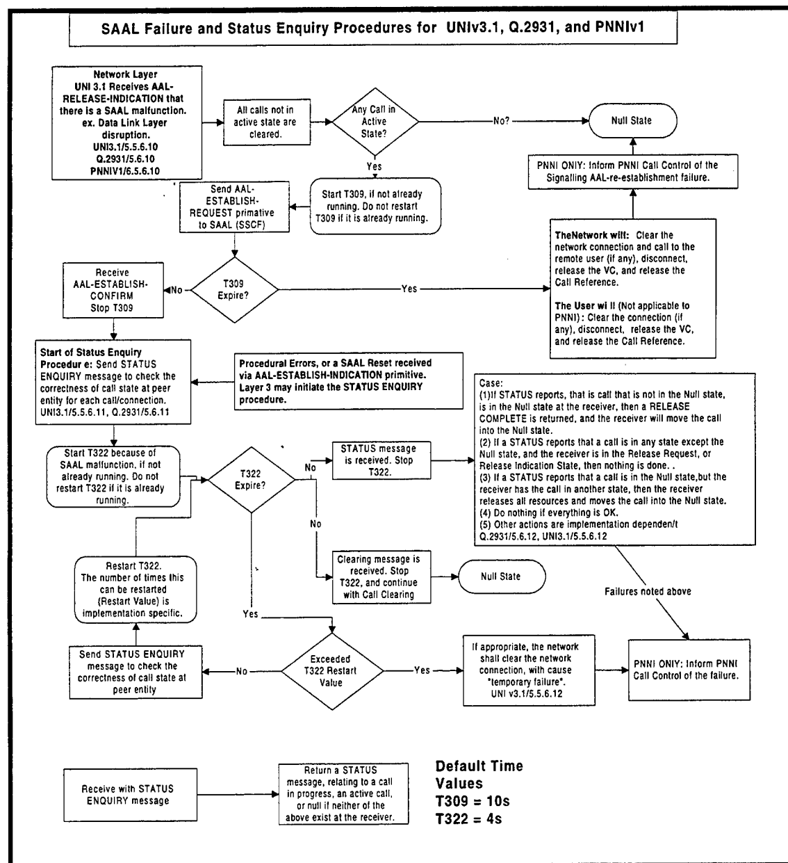
Figure 34. SAAL Failure and Status Enquiry Procedures for UNI3.1, Q.2931, and PNNI
