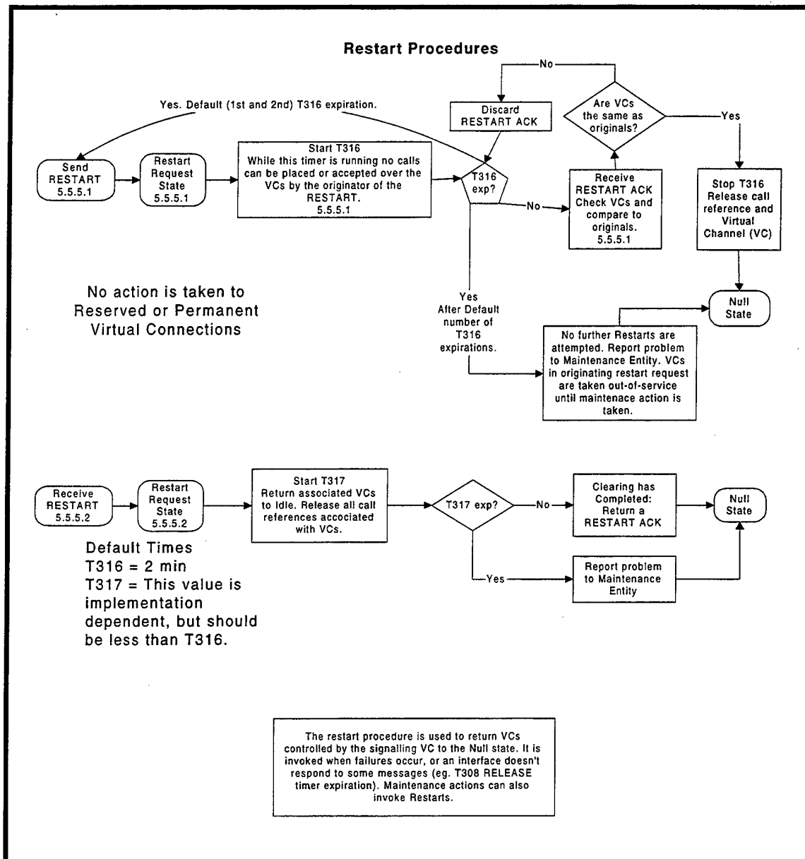
Figure 25. Control Plane – UNI 3.1 Restart Procedures
