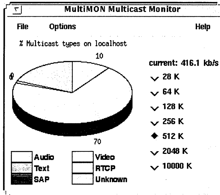
Figure 2.4 MultiMON client window (Robinson, et al, 96).
