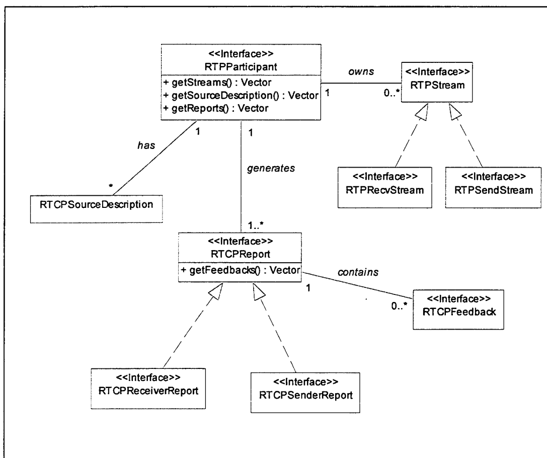
Figure 4.3 RTPParticipant Class Diagram.
