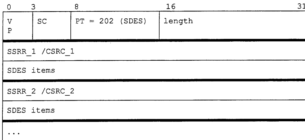
Figure 3.7 Source Description (SDES) Packet Format (Schulzrinne, et al., 99).
