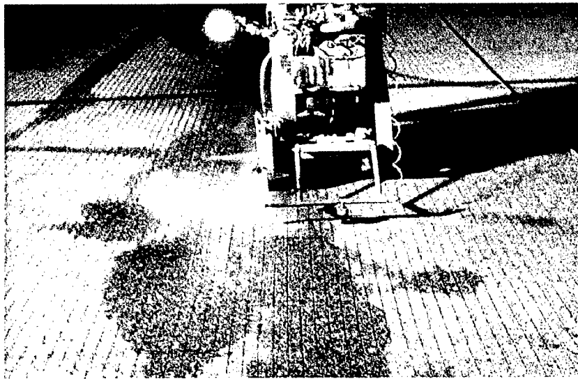
Figure 8. Saw-Cutting the Runway/Taxiway
