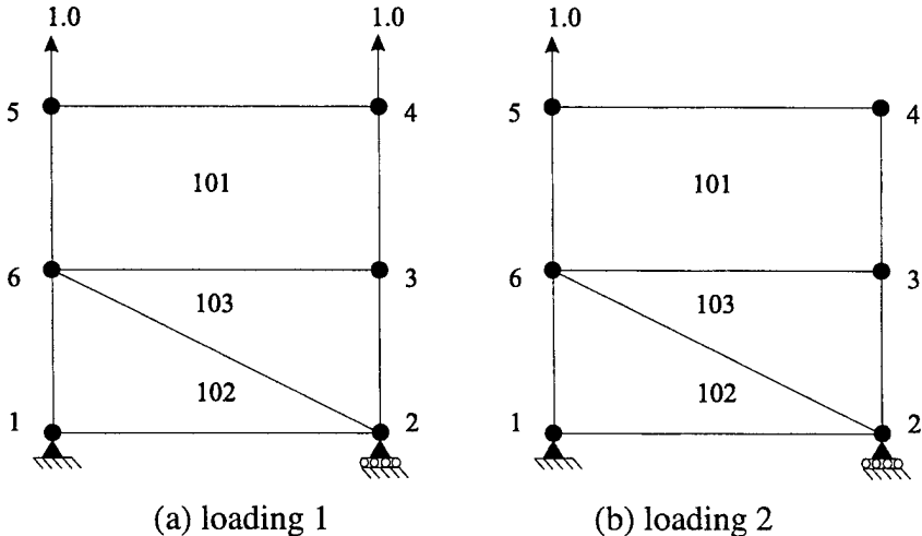
Figure 1.1: A simple FEM model
