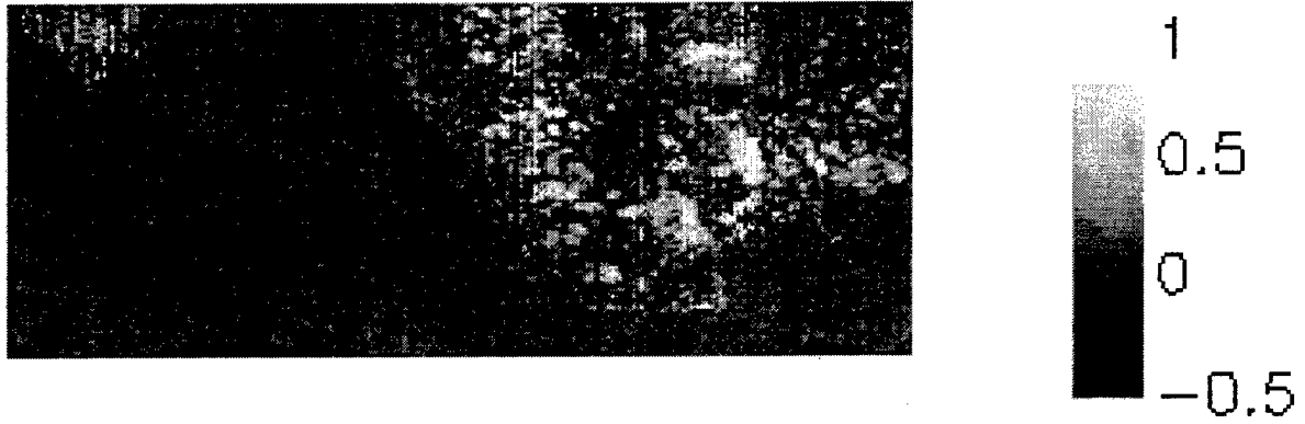
Figure 21. SMF- Vegetation Class Probability
