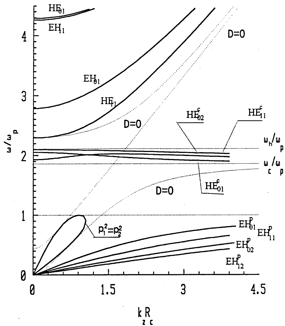
Fig.1 The typical dispersion curves with B_0=0.175T ( \omega_c/\omega_p=1.86 ), \omega_p=1.85 \times 10^{10} s^{-1} , R=1.5cm .
