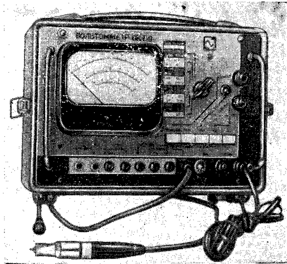
Figure 12.21.1. Exterior view of the VK7-9 voltohmmeter ("Inkrustatsiya").
