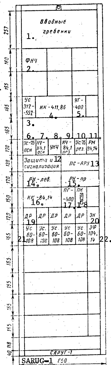
The placement of the equipment in the SARUG-1 automatic gain control rack.
