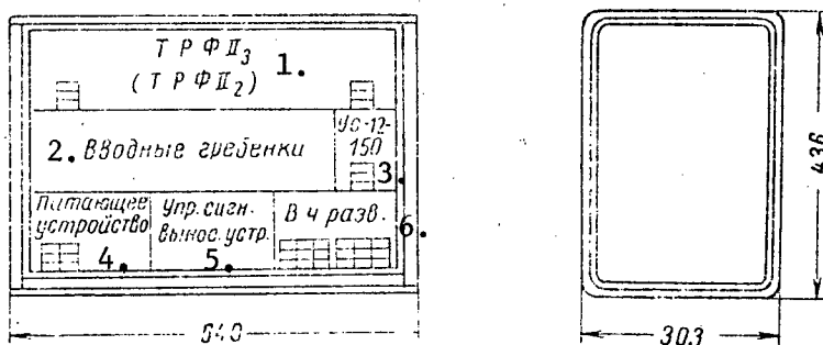
Figure 9.3.3. The placement of the equipment in the remote unit of the AV-2/3 broadcast equipment.
