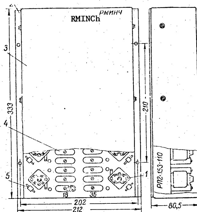
Figure 13.2.1. The construction of the RMINCh power distributor for individual carrier frequencies.
