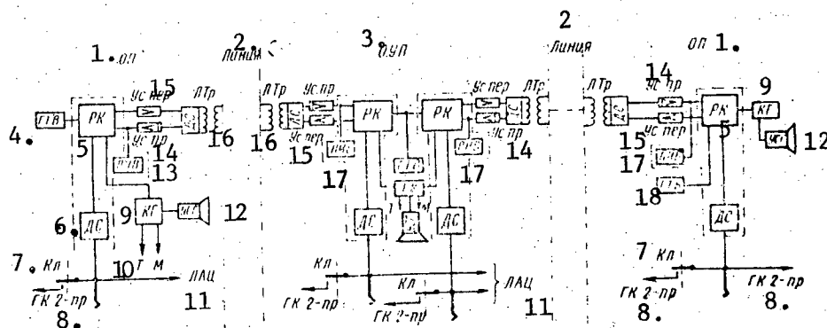
Figure 11.2.9. Block diagram of USS sectional service communications using a two-wire channel.
