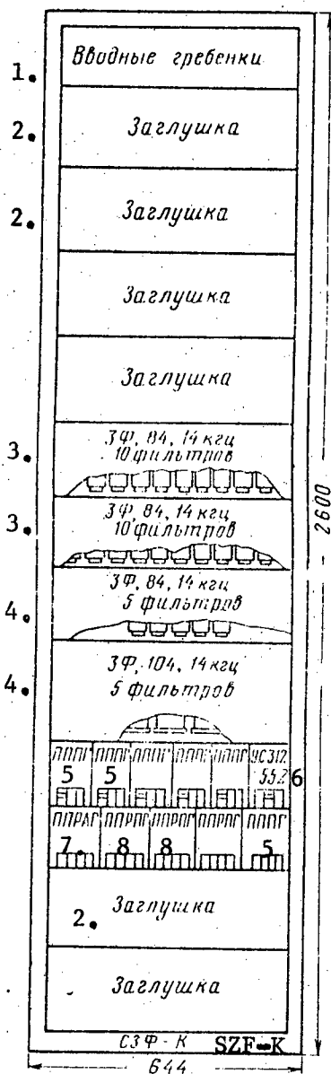
Figure 11.6.1. The placement of the equipment in the SZF-K rack of blocking filters.
