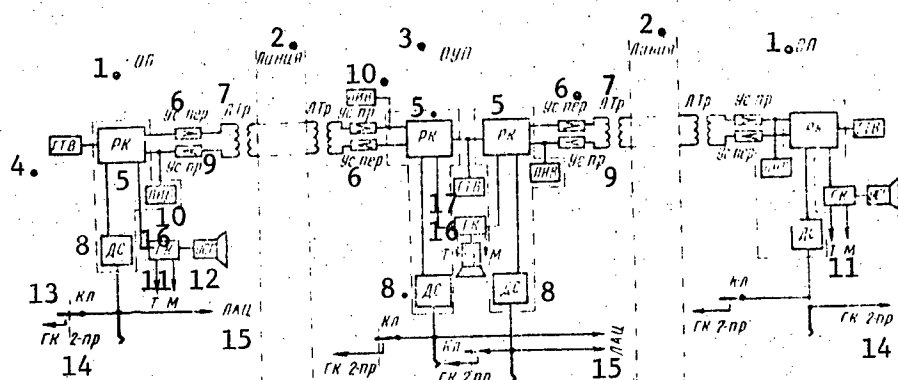
Figure 11.2.8. Block diagram of USS sectional service communications using a four-wire channel.
