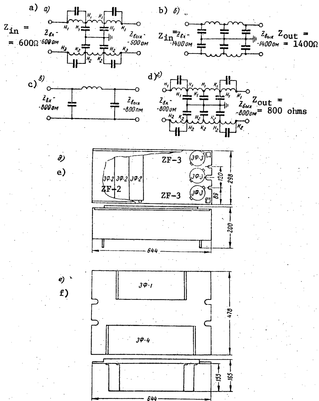
Figure 11.5.4. The schematics and construction of the ZF suppression filters:
