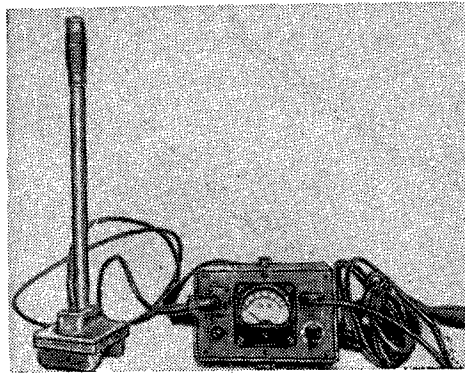
Figure 12.36.3. Exterior view of the IMP-1 finder for the location of a breakdown in cable insulation.
