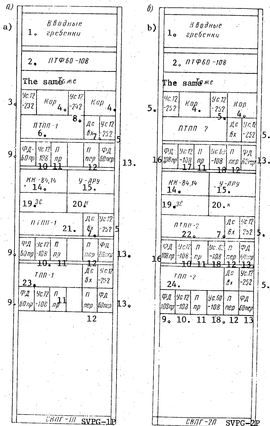
Figure 8.3.2. The equipment placement in the rack for primary group segregation: a) SVPG-1P; b) SVPG-2P.
