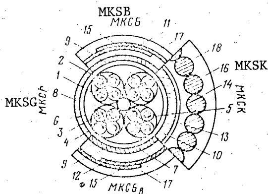
Figure A.1.1. Section through type MKS cable, 4 x 4 x 1.2.
