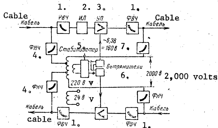
Figure 5.2.32. Block diagram of the SU-NUP amplifier rack of the K-1920 equipment.
