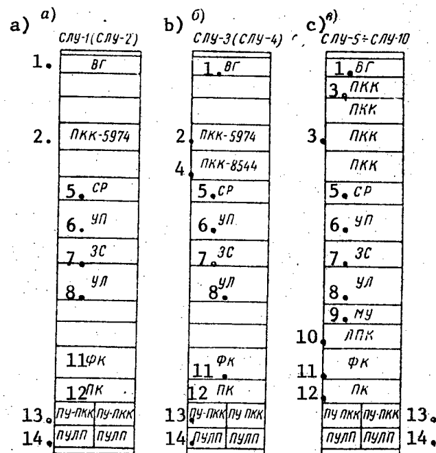
Figure 5.2.11. The placement of the panels in the following racks: a) SLU-1 (or SLU-2); b) SLU-3 (or SLU-4); c) SLU-5 -- SLU-10 of the K-1920 equipment.
