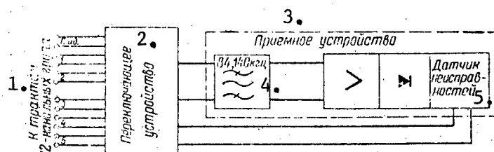
Figure 11.10.1. Block diagram of the panel for primary group monitoring.
