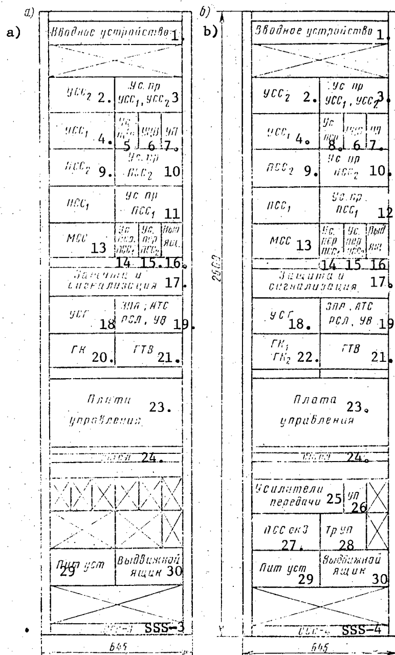
Figure 11.2.2. The placement of the equipment in the standardized service communications racks: a) SSS-3; b) SSS-4.
