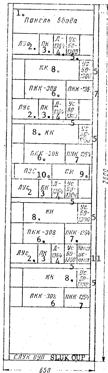
Figure 5.1.2. The placement of the equipment in the amplifier and corrective network rack, SLUK-0UP, of the K-300 equipment.
