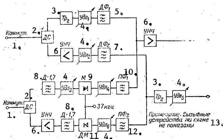
Figure 11.9.1. Block diagram of the SDK-2 channel division rack.
