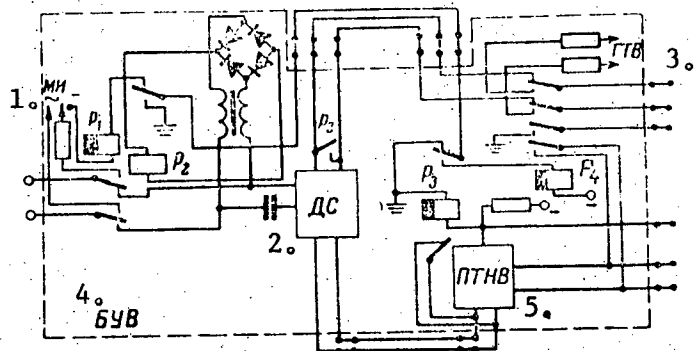
Figure 7.3.3. Schematic of the voice frequency ringing and differential system rack, STV-DS-60.
