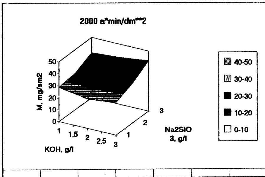
fig. 3. Response surfaces of the coating mass at values of Q = 1000 (a), 1500 (b) and 2000 (c) Amin/dm^2 .
