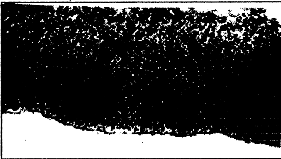
fig. 5. Micrographs of cross sections of oxide ceramic coatings produced in 2 g/l KOH + 2 g/l Na 2 SiO 3 electrolyte at Q = 300 (a); 630 (b) and 2000 (c) Amin/dm 2 . Mag. x450x4.
