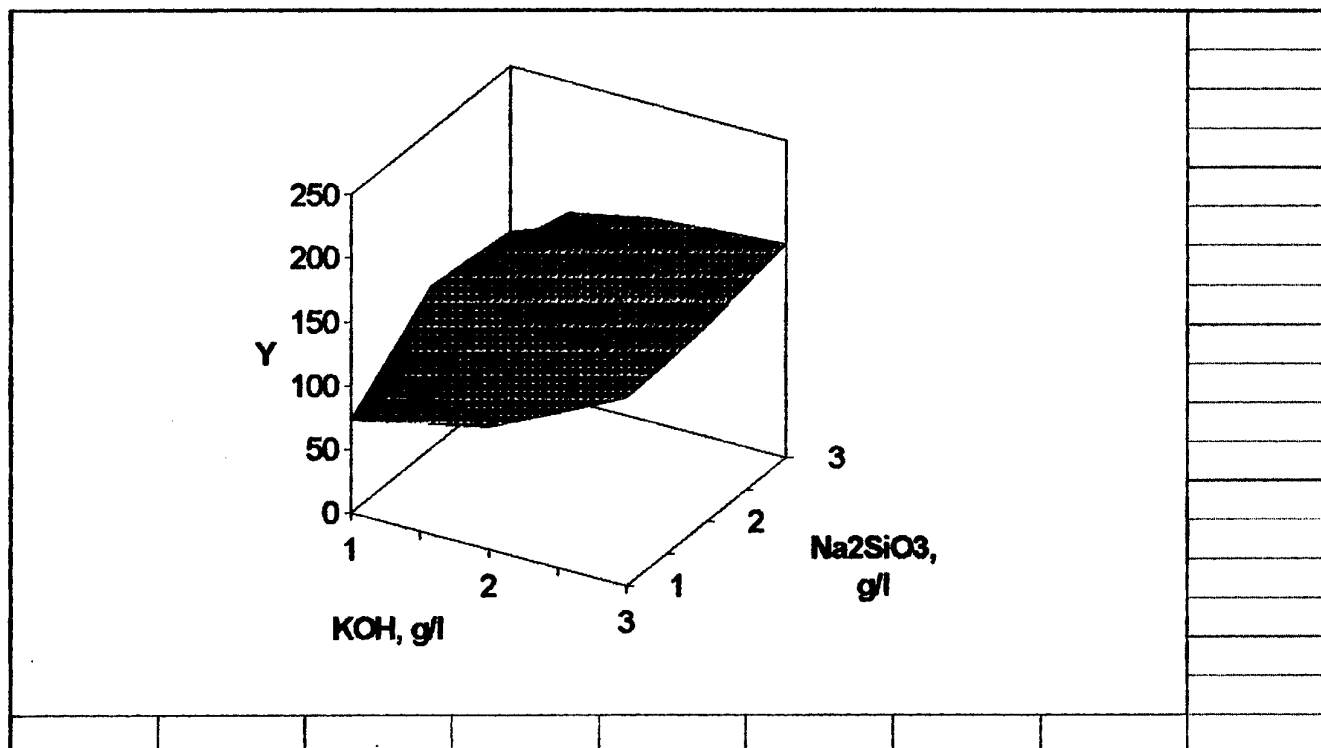
fig 8. Response surface for generalized optimizing parameter Y of MDO process at top level of factor Q.
