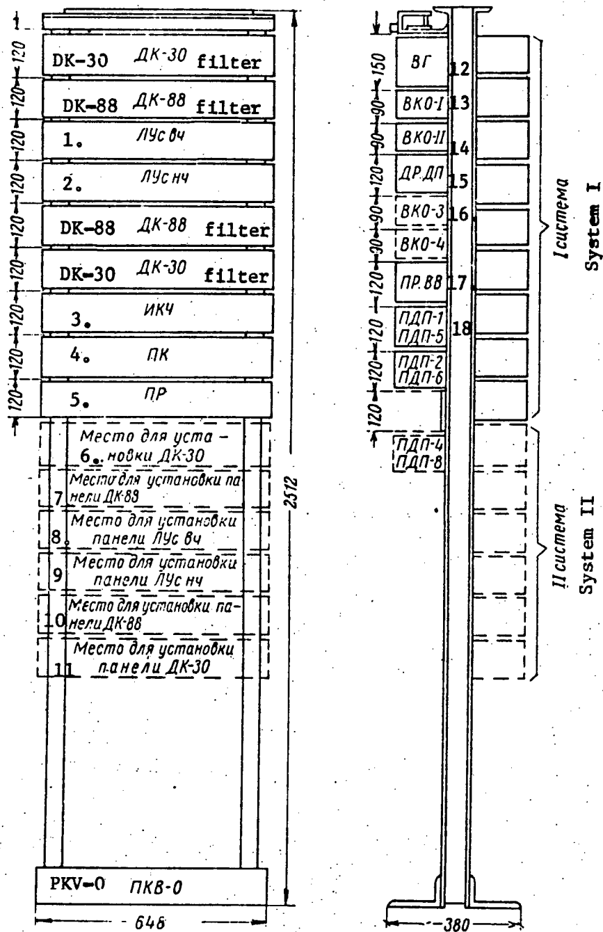
Figure 4.3.3. The placement of the equipment in the PKV-0 attended intermediate amplifier station of the KV-12 equipment for 1 - 2 systems.
