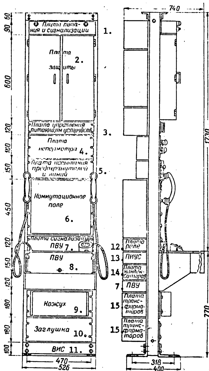
Figure 1.2.2. The equipment layout in the VIS input-test rack.
