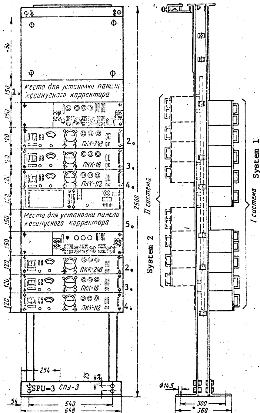
Figure 4.7.9. The placement of the equipment in the rack of intermediate amplifiers with three-frequency AGC, the SPU-3, of the K-60 equipment.
