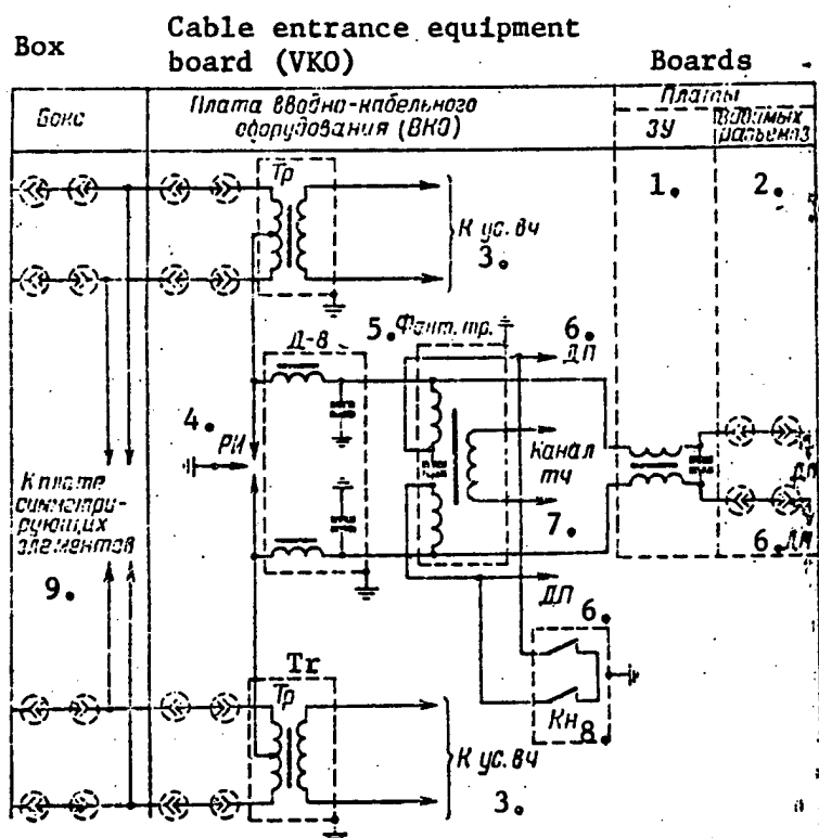
Figure 1.13.10. Schematic of the VKS-OUF rack [cable entrance rack--attended repeater station].
