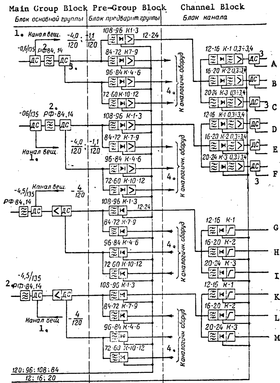
Figure 4.5.5. [Second half of Figure on page 288] Block diagram of the SIO individual conversion equipment rack of the BK-24 equipment. The jumpers are removed when working through a four-wire circuit.
