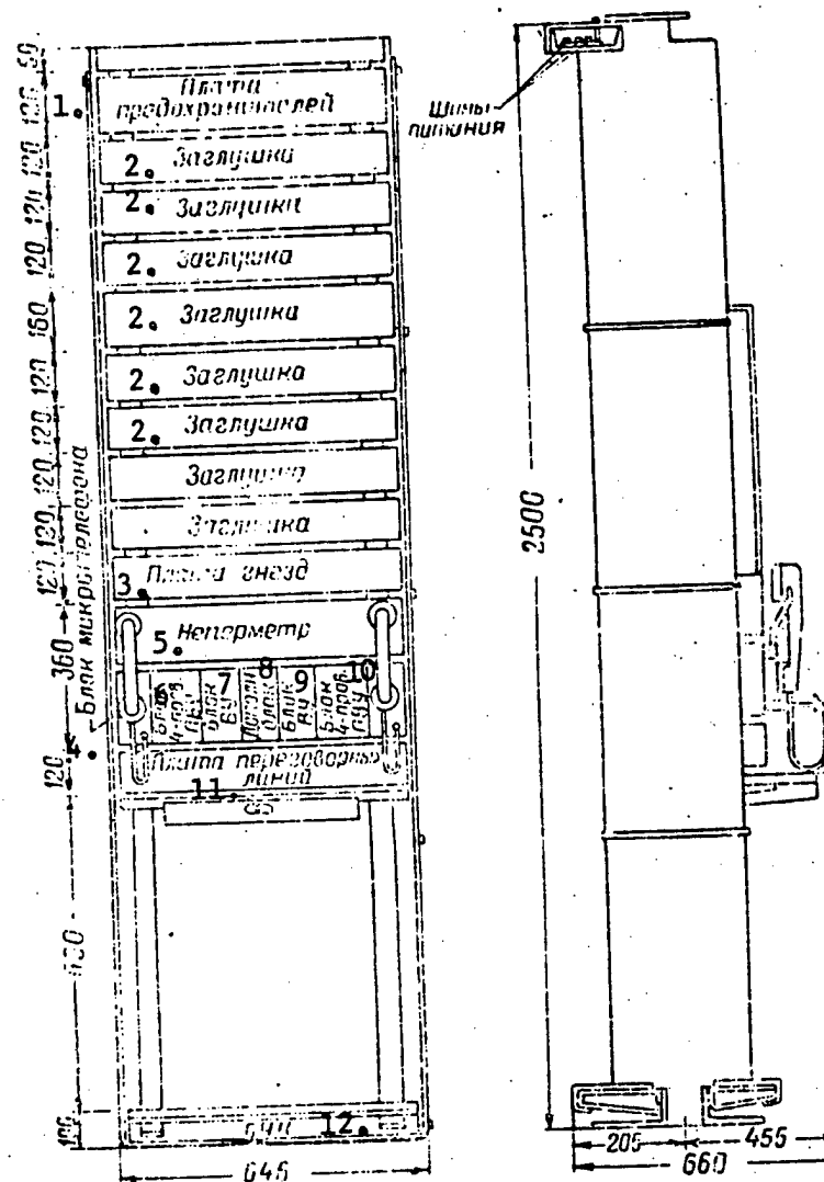
Figure 1.11.2. The equipment layout in the SChK four-wire switching rack.
