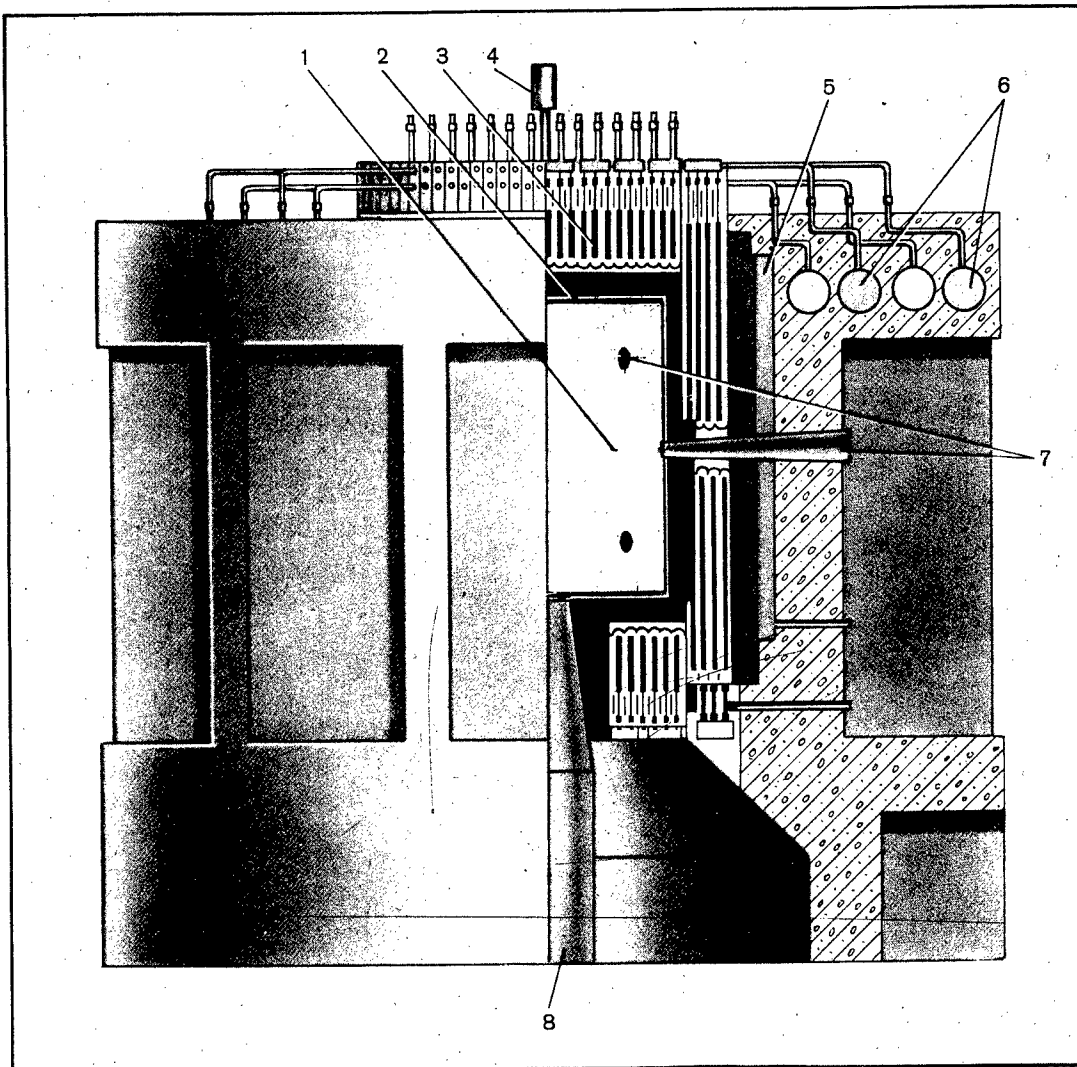
Design of the hybrid laser-driven fusion reactor: 1--explosion chamber; 2--porous wall; 3--cartridges with uranium (blanket); 4--port for introducing the target; 5--tritium breeding zone (lithium); 6--coolant (helium) circulation loop; 7--ports for laser emission; 8--vacuum port
