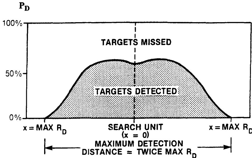
Figure 2-2. Typical lateral range curve.
