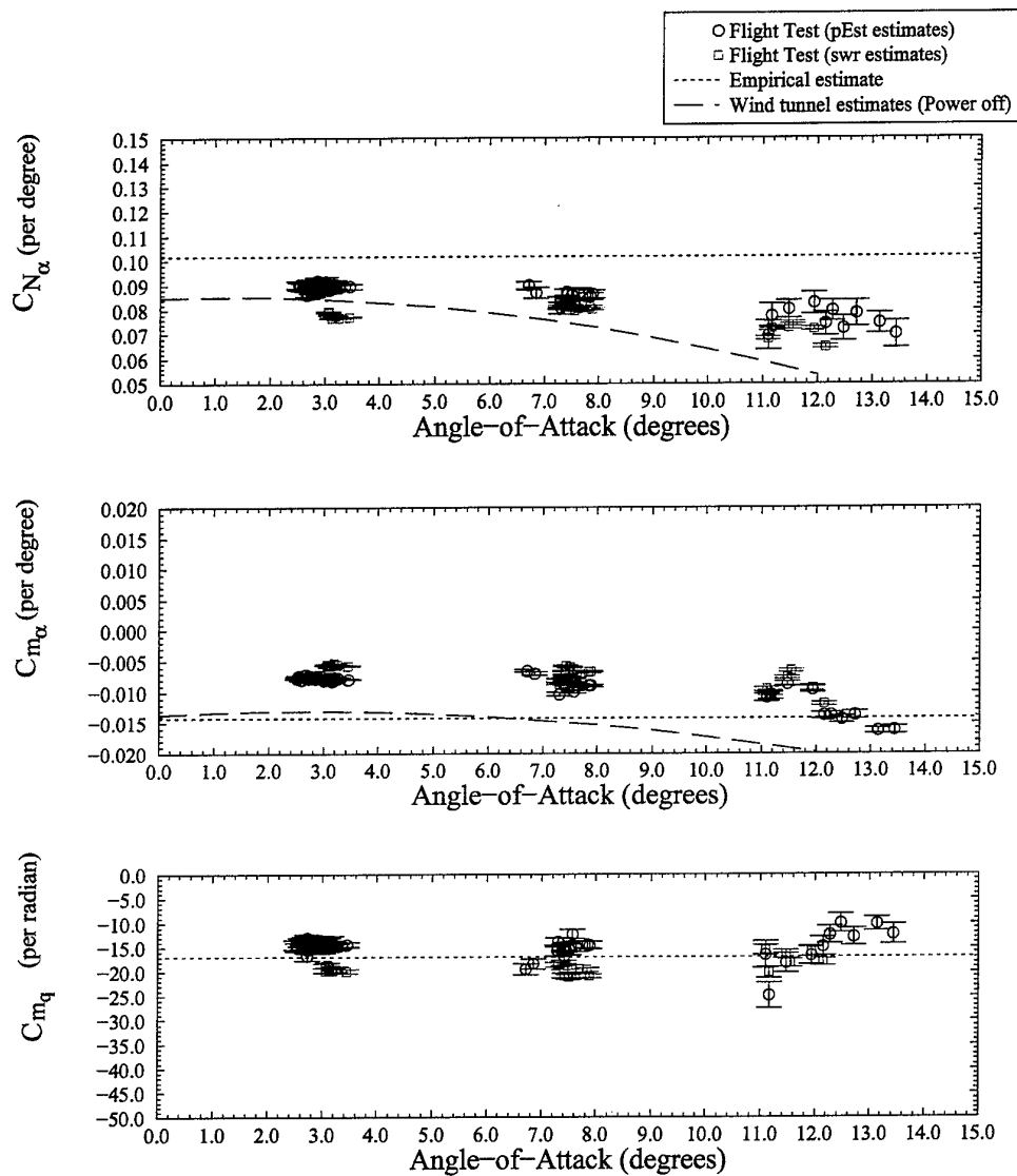
Figure 2: PC 9/A angle-of-attack and pitch rate derivatives, 3-2-1-1 manoeuvres at 5000 ft.
