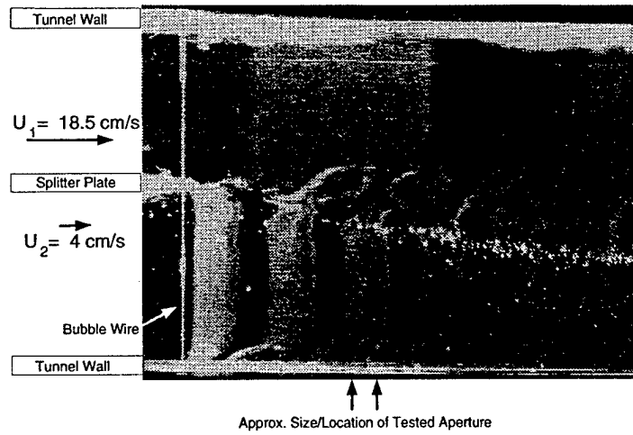
Figure 15. Hydrogen bubble visualization of heated mixing layer (looking up through the bottom of tunnel test section).
