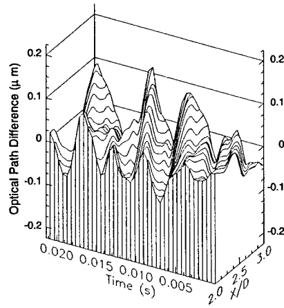
Figure 2. Space-time representation of SABT-measured OPDs for propagation through an experimental, two-dimensional, heated jet flowfield (from Ref. 6).
