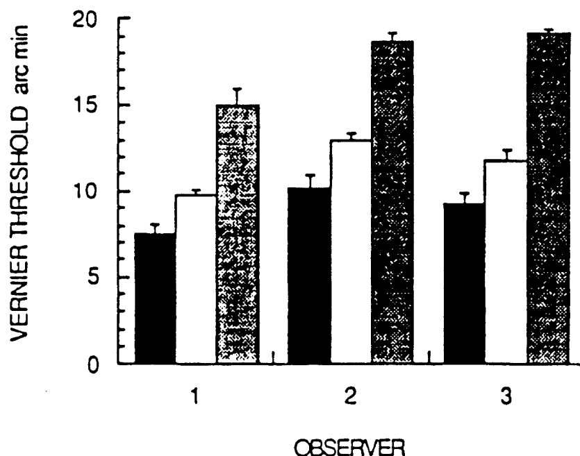
Figure 3. Vernier step acuity thresholds for boundaries defined by combinations of orientation contrast ( \beta ) and luminance contrast ( C ). Black bars: \beta = 70 deg, C = 20\% . White bars: \beta = 70 deg, C = 0\% . Gray bars: \beta = 0 deg, C = 20\% .
