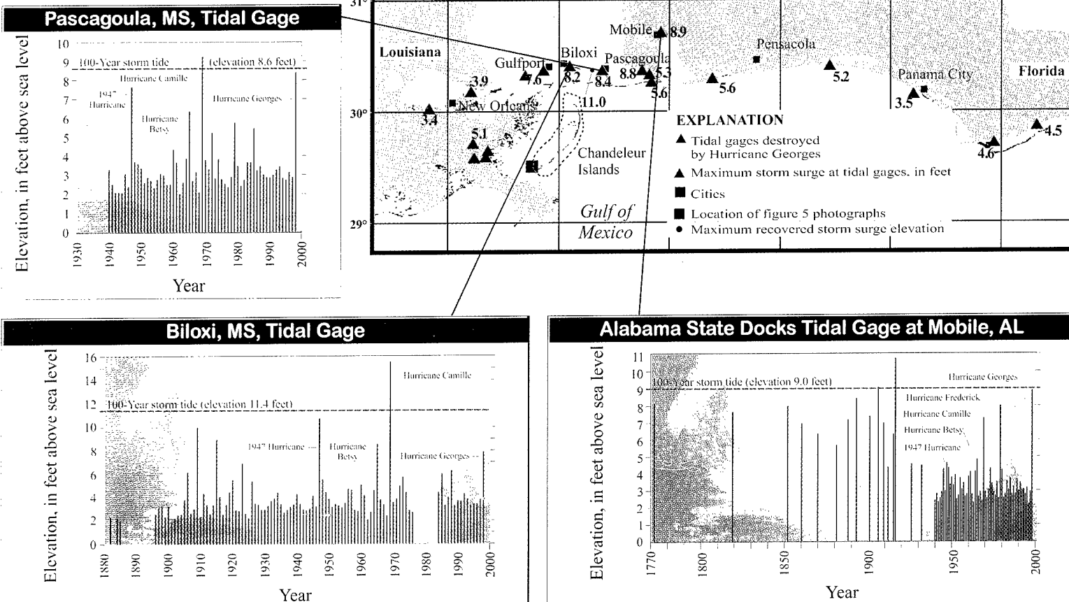
Figure 4. Location of selected provisional tidal surge elevations caused by Hurricane Georges in Louisiana, Mississippi, Alabama, and Florida, and annual maximum tidal stages for three selected U.S. Army Corps of Engineers tidal gages.
