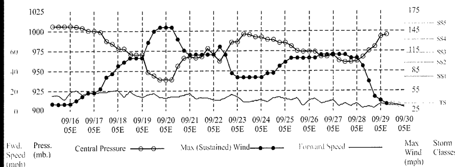
Figure 1. Central barometric pressure (in millibars), maximum sustained wind and forward speed (in miles per hour) for Hurricane Georges from September 16 through 30, 1998. (Courtesy of NOAA/NW Southeast River Forecast Center)
