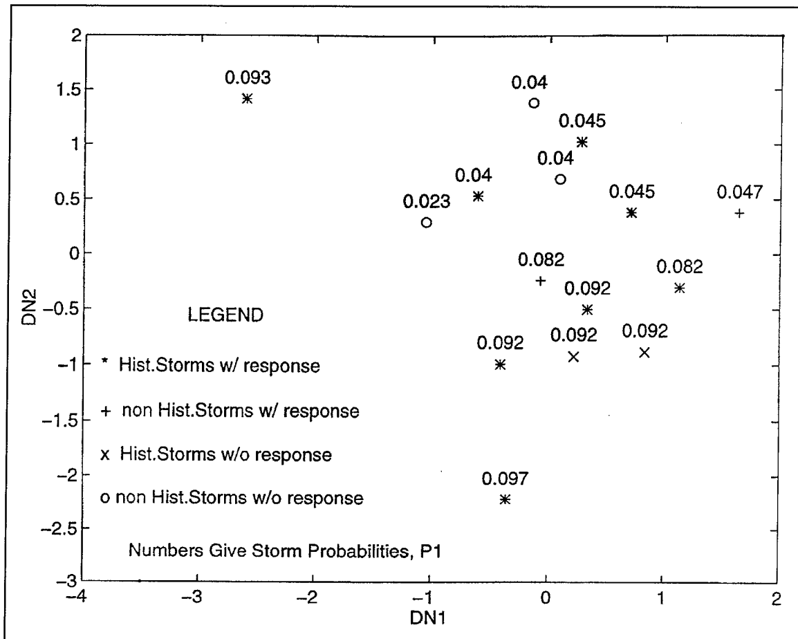
Figure 11. Enhanced probabilities
