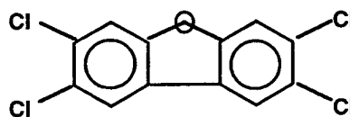
Chlorinated Dibenzofurans (135 congeners)
