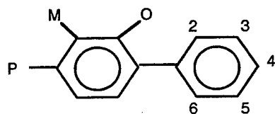
Polychlorinated biphenyls (209 congeners)
