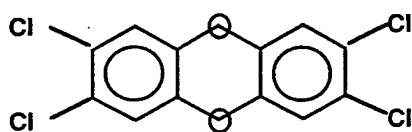
Chlorinated Dibenzodioxins (75 congeners)
