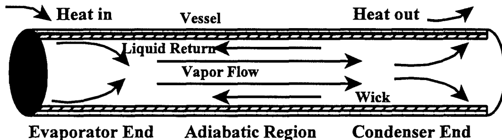
Figure 4. Basic Heat Pipe Configuration
