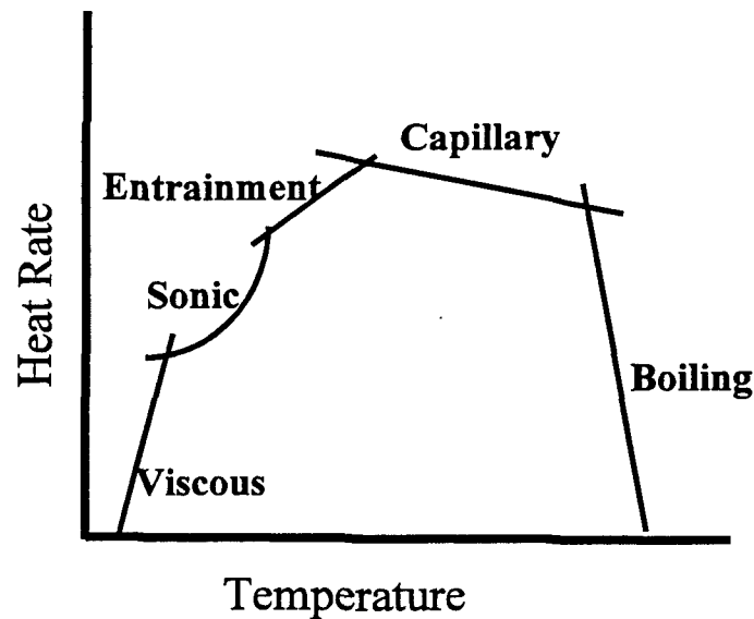
Figure 6. Heating Limits
