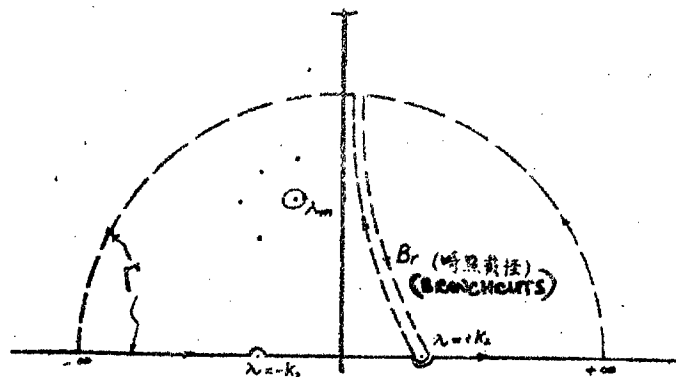
Diagram 3. \lambda -surface Integral Curve.
