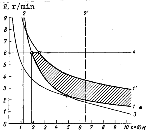
Graphic illustration of system of inequalities (8)
