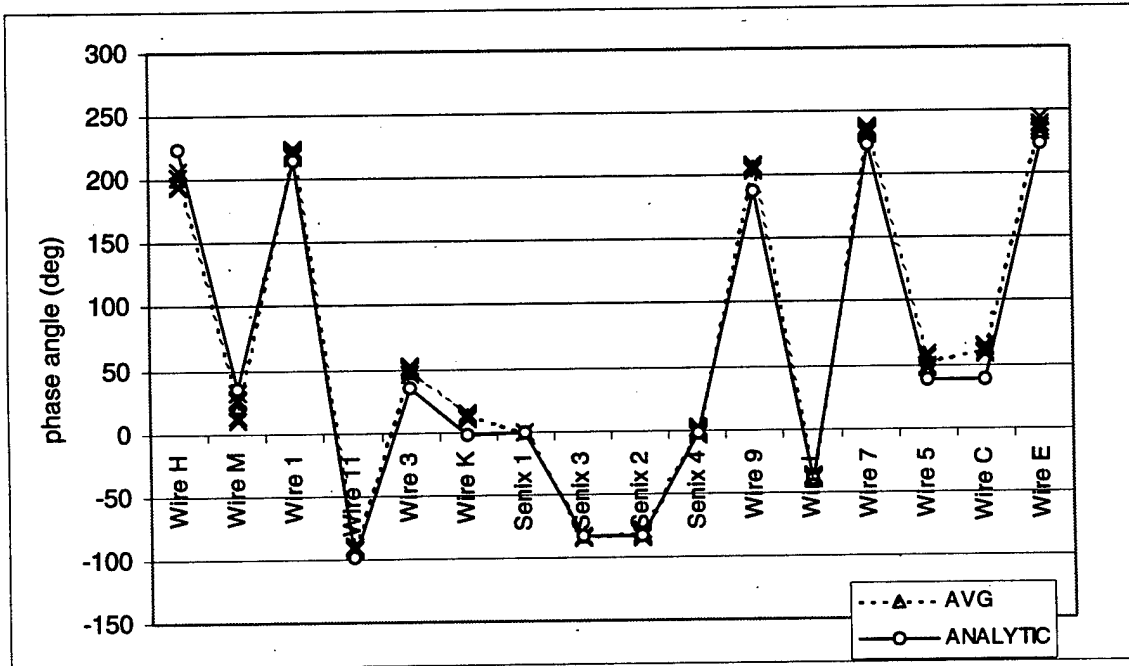
Figure 21. Wave phase angle by probe for 2.06 second period from 'A' bank.
