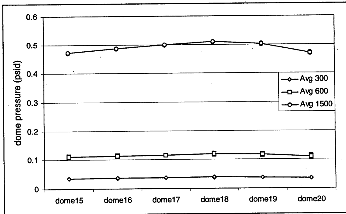
Figure 41. 'B' bank dome pressure for 1.81 second period at various blower speeds (rpm).
