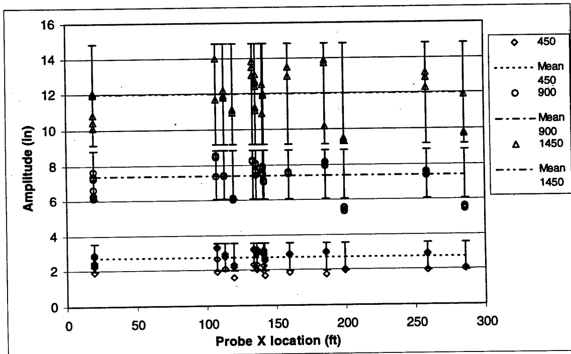
Figure 17. Wave amplitude by probe location and blower speed (rpm) at 3.1 seconds on 'B' bank.
