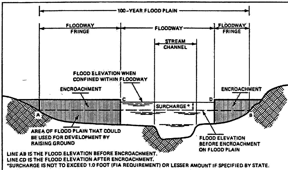
Figure 2 - Floodway Schematic
