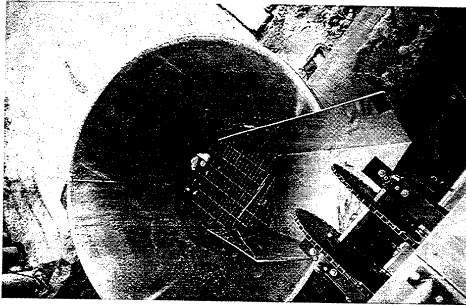
Figure 9 Shuttle box dump to open grate furnace
