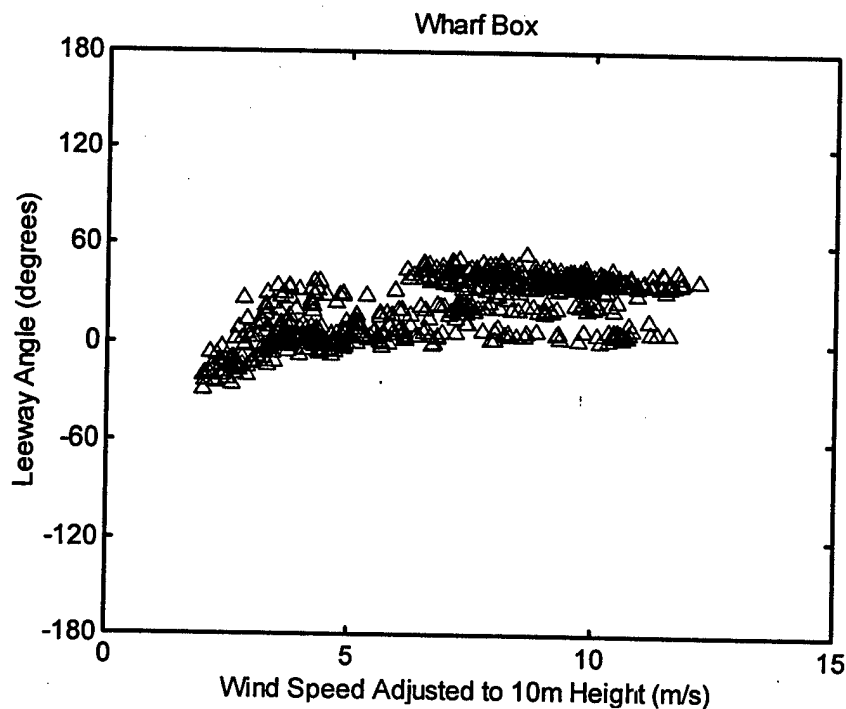
Figure 4-19. Leeway Angle (degrees vs. 10m Wind Speed (m/s) for the Wharf Box with One and Four-person Loads
