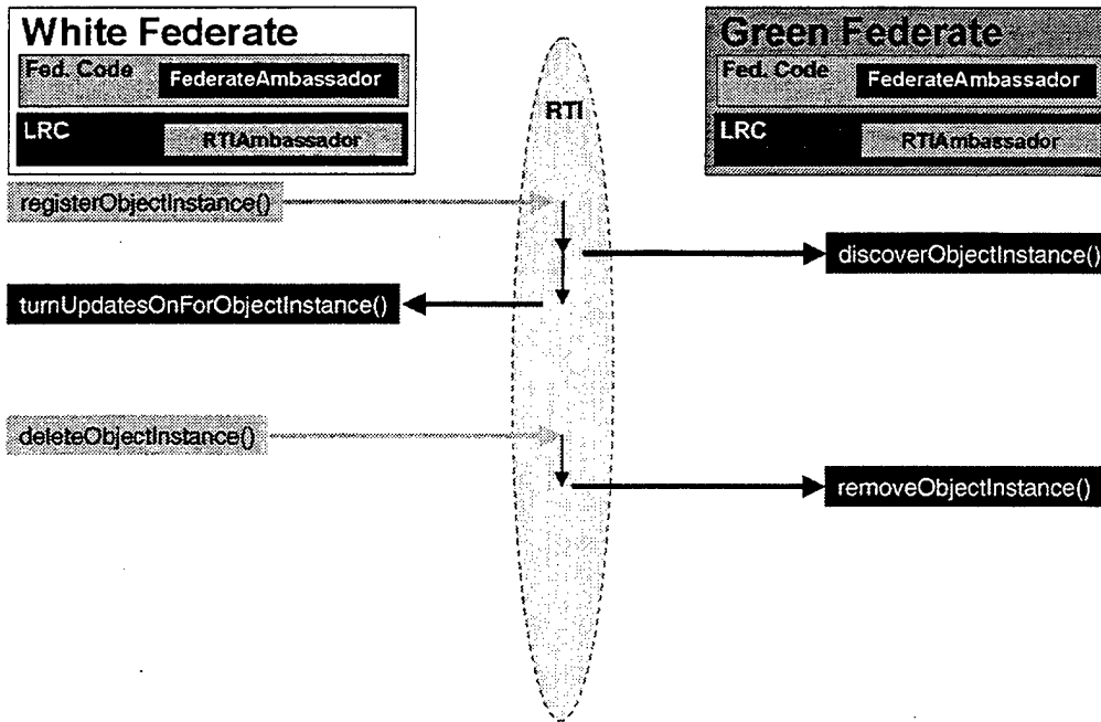
Figure 12. Registering, Discovering, and Deleting Object Instances. [From Ref 4].
