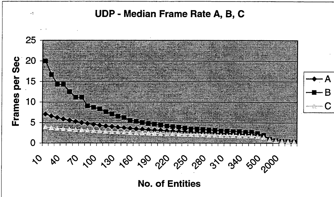
Figure 21. UDP – Median Frame Rate for Systems A, B, and C.
