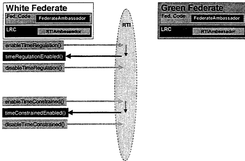
Figure 6. Toggling Regulating and Constrained Status. [From Ref. 4].
