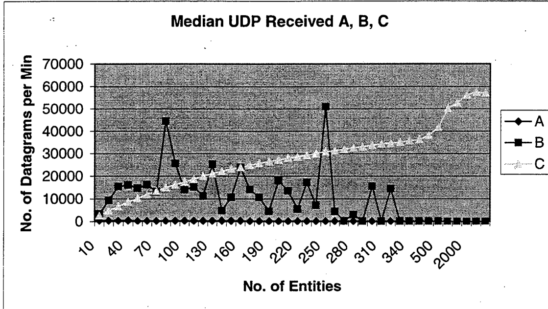
Figure 29. Median UDP Received for Systems A, B, and C.
