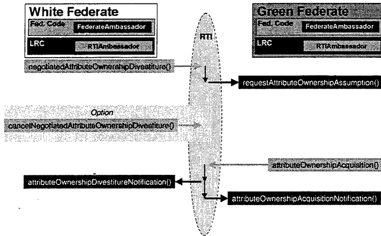
Figure 17. Pushing Ownership To Other Federates. [From Ref. 4].
