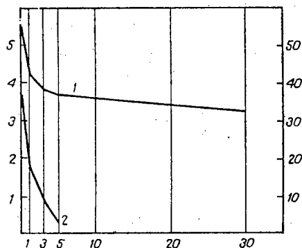
Change in COU (1) and intensity of odor (2) of ozone-treated liquid waste. X-axis, time of observation (days); y-axis, odor (graded in points), on the left; COU (mg/l), on the right.
