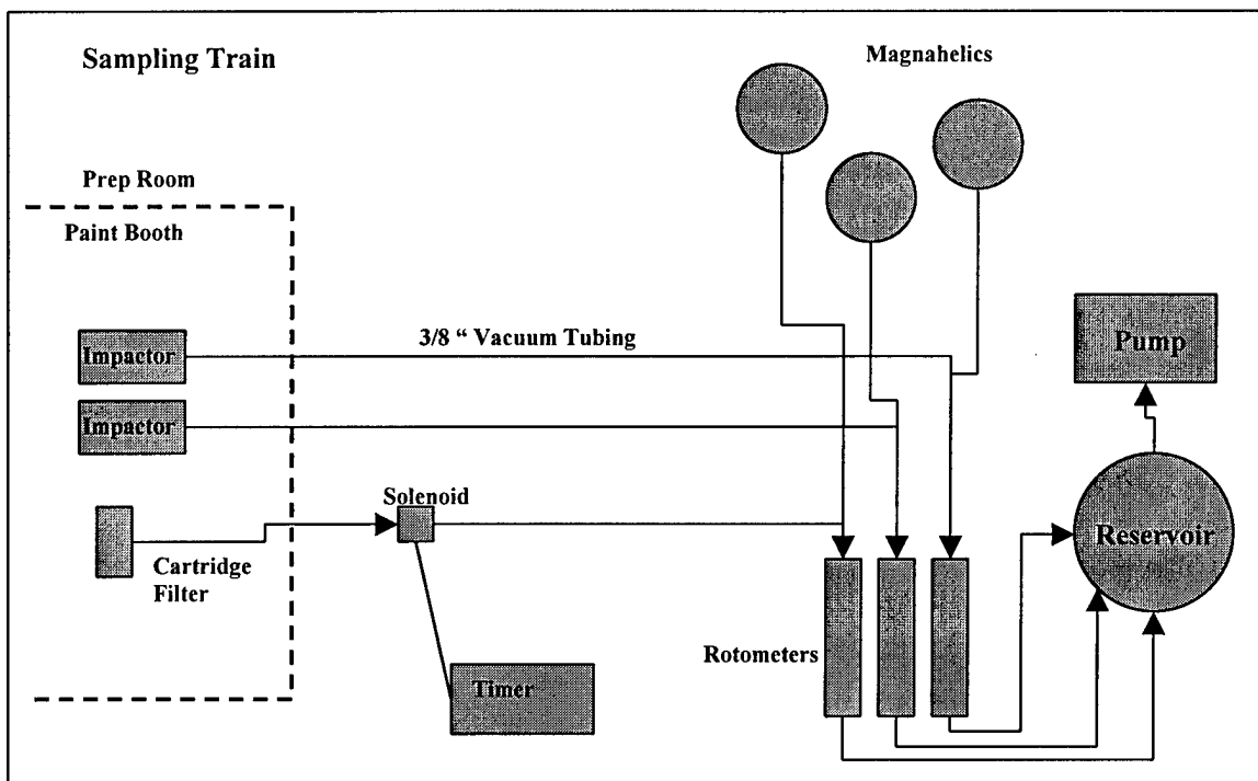
Figure 5. Sampling Train
