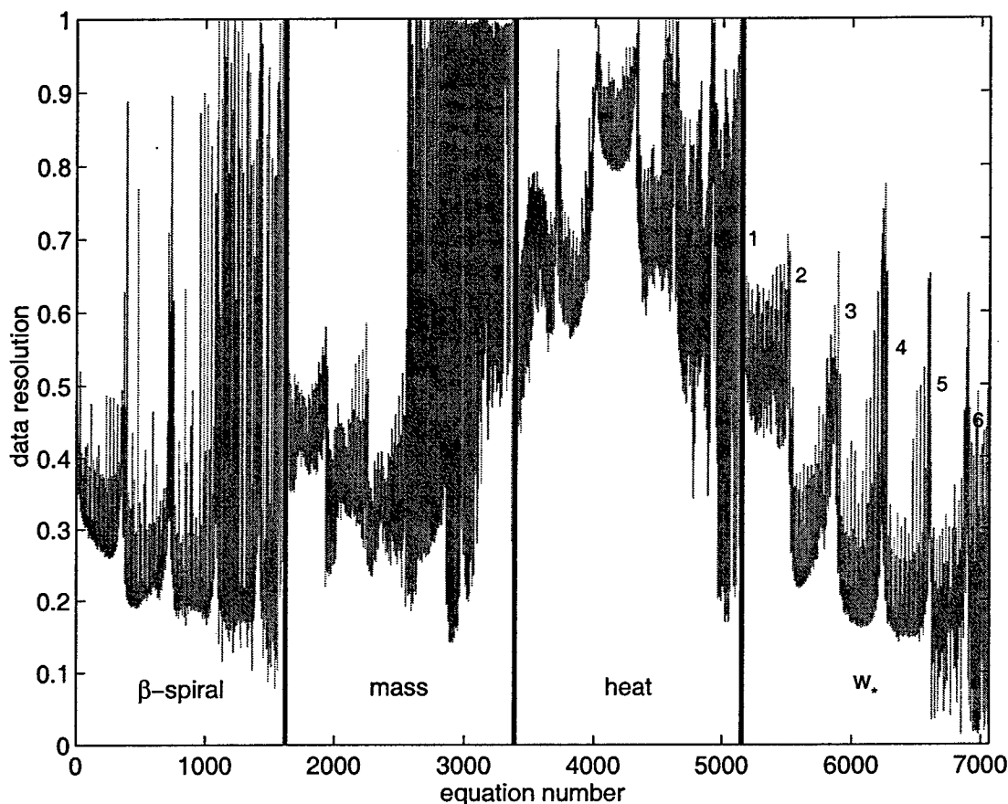
Figure 3.9: The diagonal elements of the data resolution matrix. The four classes of model equations are ordered by equation number. For each equation class, increasing equation numbers correspond to deeper layers of the inverse geometry, and groups of equations for a particular layer are associated with the modulated structure of the data resolution matrix. Values of data resolution near unity indicate that equations are contributing independent information to the inversion, while lesser values signify a reduction in an equation's individual influence on the solution. \beta -spiral, mass and heat (thermal advection) equations all contribute strongly to estimates of deep flow. The influence of the diapycnal advection constraints is reduced in successively deeper layers, as numbered 1-6.
