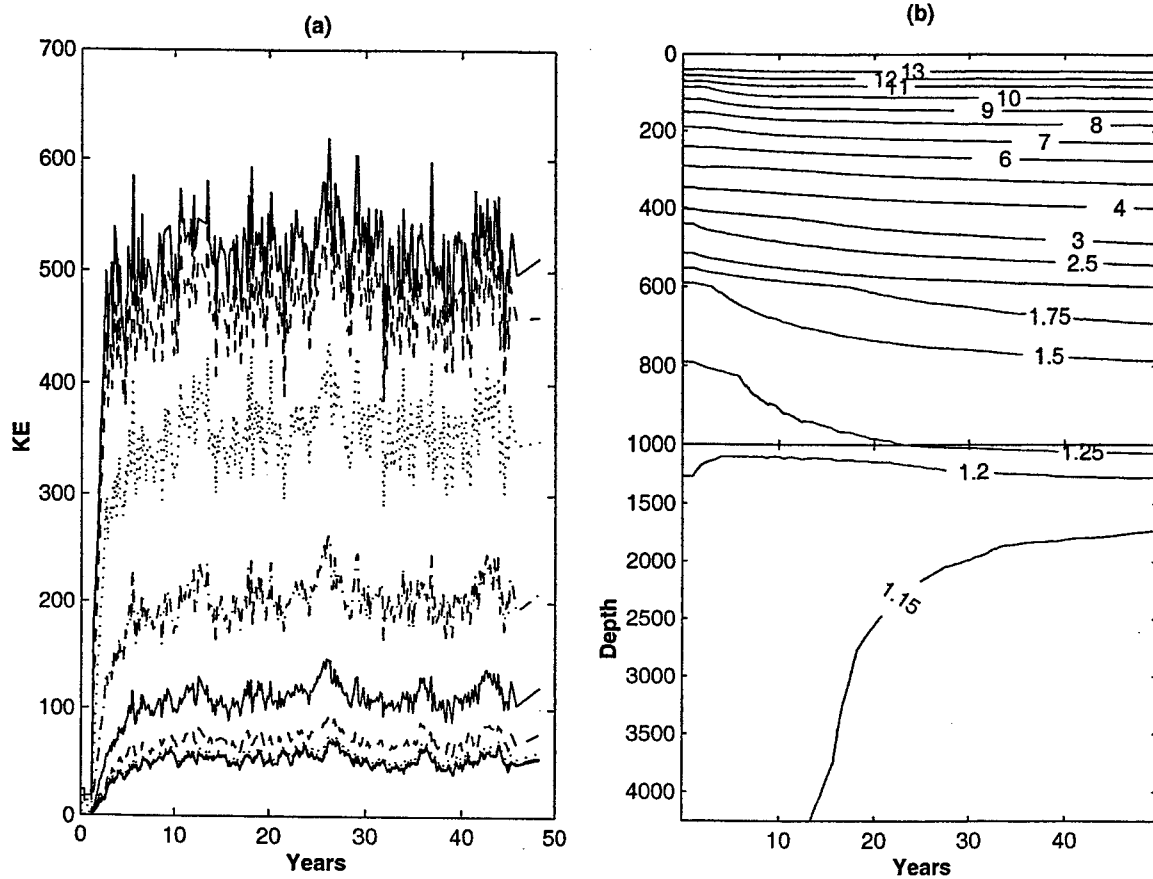
Figure 2-6: Spin-up stage of the eddy resolving simulation: (a) horizontal kinetic energy for each layer (upper layers at the top), (b) horizontally averaged temperature. Note: upper 1000M are stretched and varying contour intervals.
