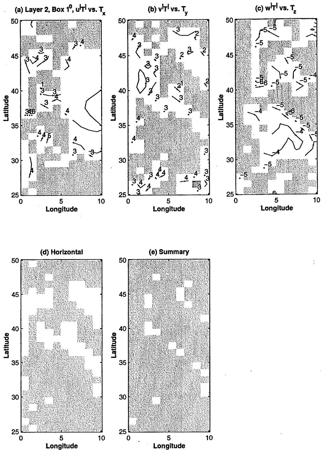
Figure 5-13: Test of the Fickian diffusivity on the 1^\circ \times 1^\circ grid. Layer 2. (a) K_{Tu} , (b) K_{Tv} , (c) K_{Tw} , (d) horizontal test, (e) summary of the test. White areas identify the positive diffusivity coefficients. Contour values are \log_{10} of the coefficients, [M^2 \cdot \text{sec}^{-1}] .
