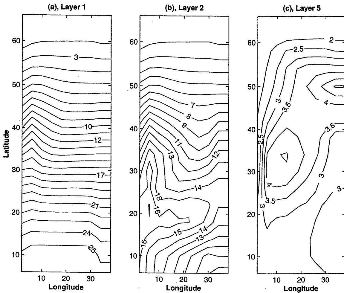
Figure 2-3: Temperature fields [ ^{\circ}\text{C} ] used in the initialization procedure: (a) upper surface layer, (b) second sub-surface layer, (c) 5 th thermocline layer.
