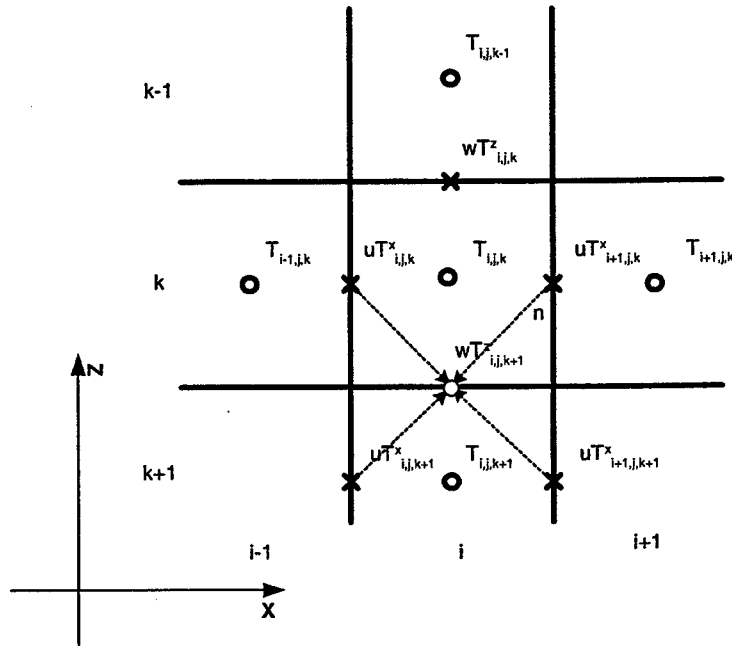
Figure 5-1: Definition of the reference point for a flux vector for an individual volume (i, j, k) in (X, Z) plane.
