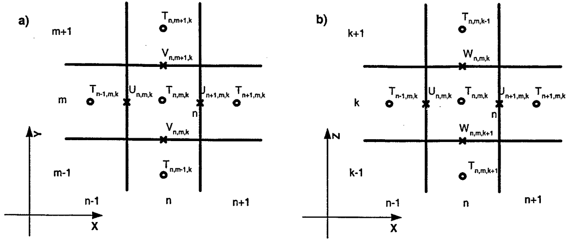
Figure B-1: Definition of the model grid in the horizontal (a) and vertical (b) planes: u, v, w - face quantities, T - zone quantity.
