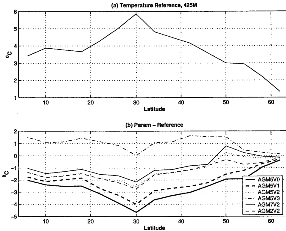
Figure 6-20: Zonally averaged temperature, section at 425M, [°C]. Gent-McWilliams Scheme. (a) Reference experiment. (b) Parameterization experiments minus Reference. Labels identify experiments.
