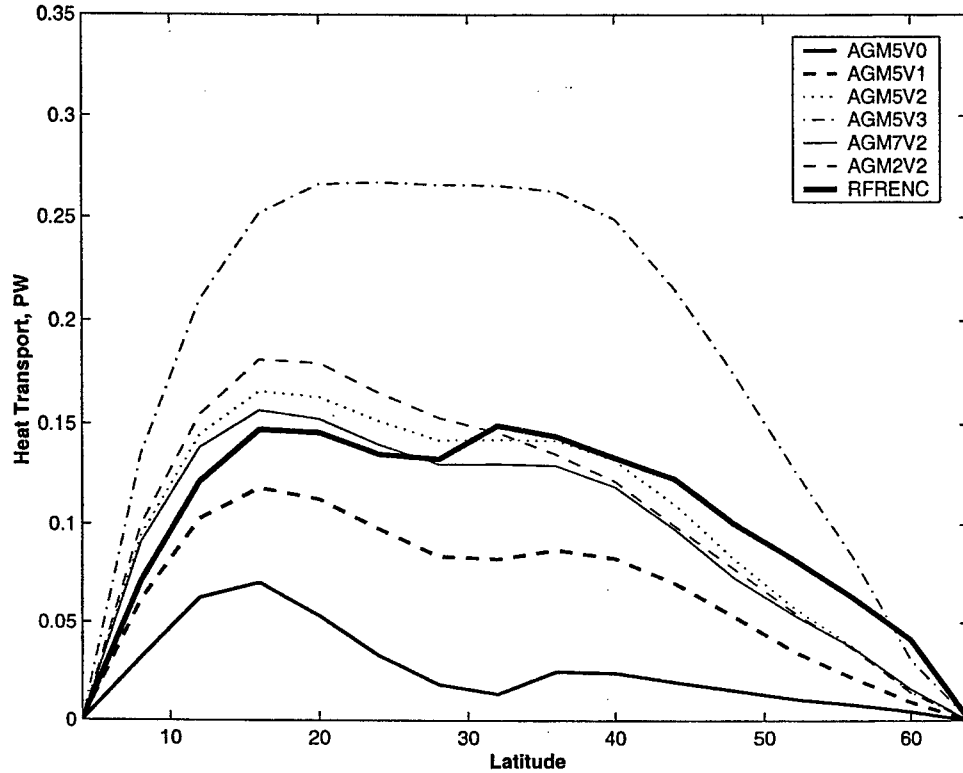
Figure 6-21: Total heat transport, [PW] . Gent-McWilliams scheme. Labels identify experiments. RFRENC is the reference experiment.
