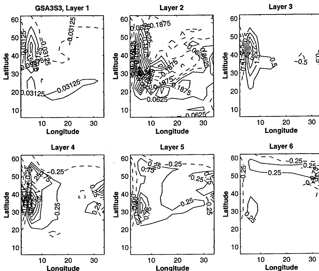
Figure 6-18: Flux divergence. Green-Stone scheme. Experiment GSA3S3 ( \alpha = 0.1 , \max(\hat{s}_{IS}) = 10^{-4} ). Layers 1 to 6. Variable C.I. in 10^{-8} [^{\circ}\text{C} \cdot \text{sec}^{-1}] units.
