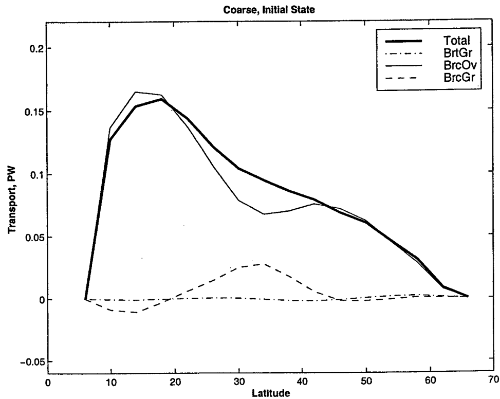
Figure 3-16: The decomposition of the total integrated northward heat transport ( Total ) of the initial state into heat transport by the barotropic gyre ( BrtGr ), baroclinic overturning ( BrcOv ) and baroclinic gyre ( BrcGr ) components, [PW].
