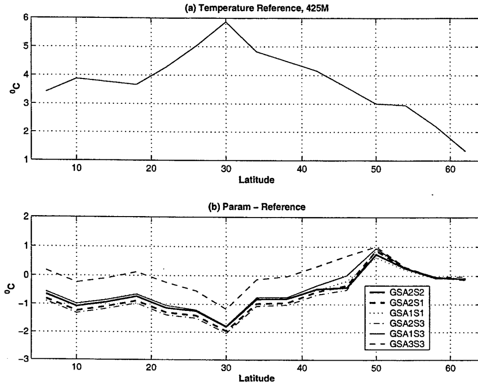
Figure 6-12: Zonally averaged temperature, section at 425M, [ ^{\circ}\text{C} ]. Green-Stone scheme. (a) Reference experiment. (b) Parameterization experiments minus Reference. Labels identify experiments.
