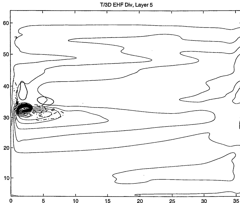
Figure 4-18: 3D divergence of the eddy heat flux, C.I. 10^{-7} [^{\circ}C \cdot \text{sec}^{-1}] , and isotherms of time-mean temperature, C.I. 1 [^{\circ}C] . Layer 5.
