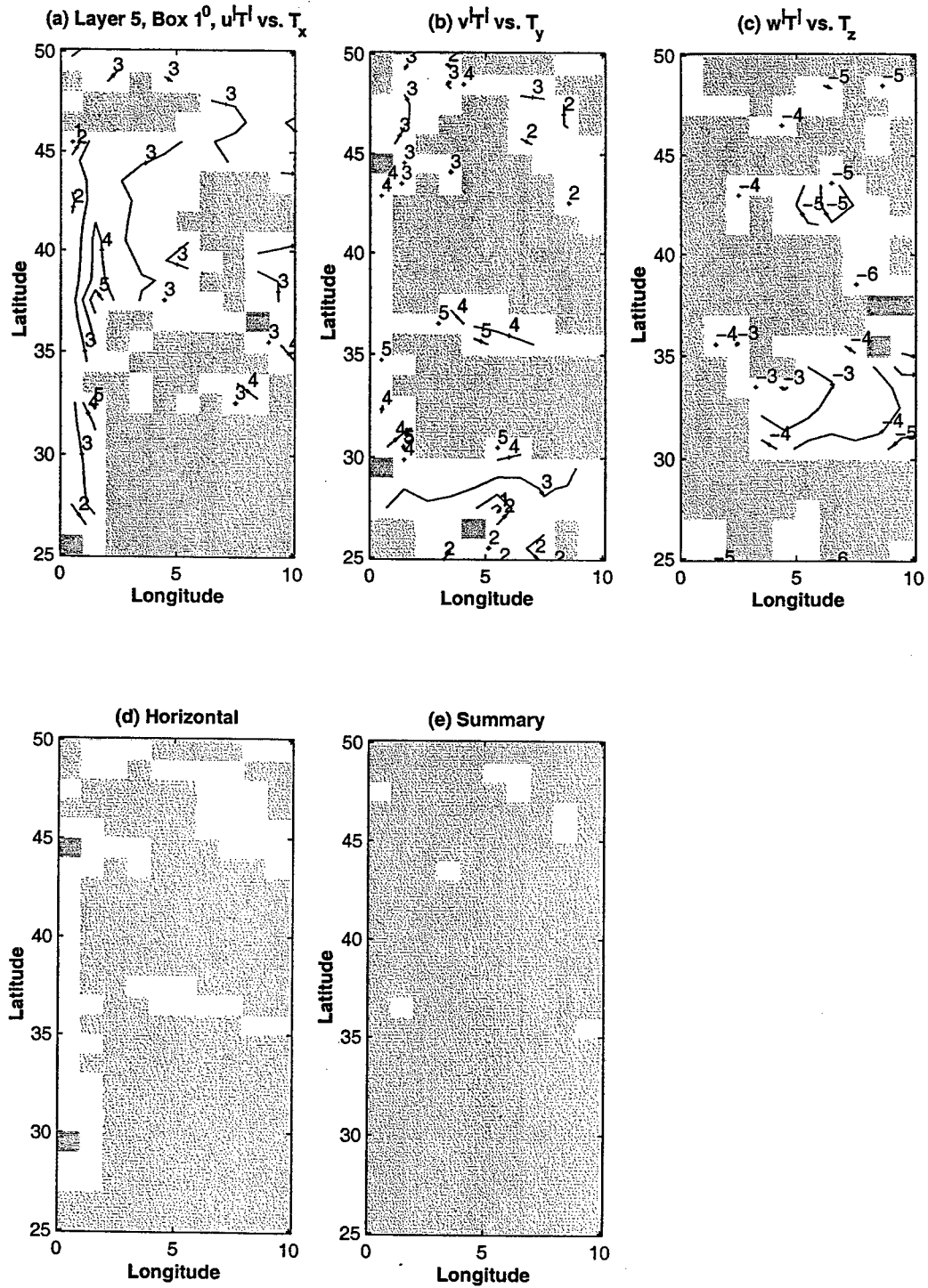
Figure 5-14: Test of the Fickian diffusivity on the 1^\circ \times 1^\circ grid. Layer 5. (a) K_{Tu} , (b) K_{Tv} , (c) K_{Tw} , (d) horizontal test, (e) summary of the test. White areas identify the positive diffusivity coefficients. Contour values are \log_{10} of the coefficients, [M^2 \cdot \text{sec}^{-1}] .
