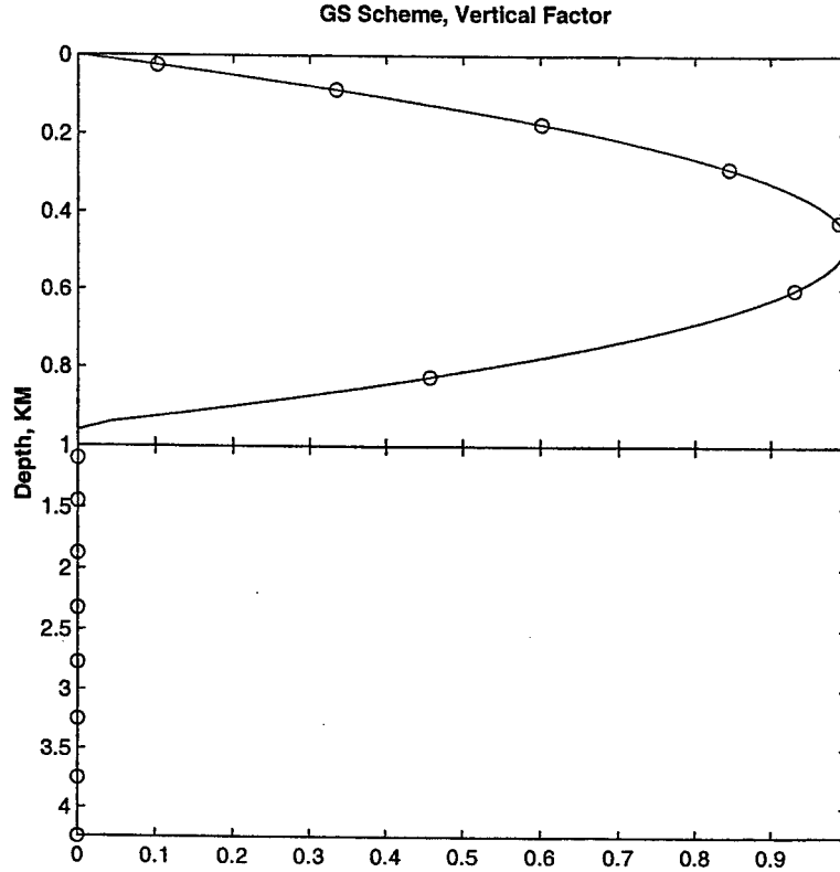
Figure 6-9: Coefficient of the vertical dependence of K_{vs} . Each circle represents the value for its respective layer. Stretched upper 1000M .
