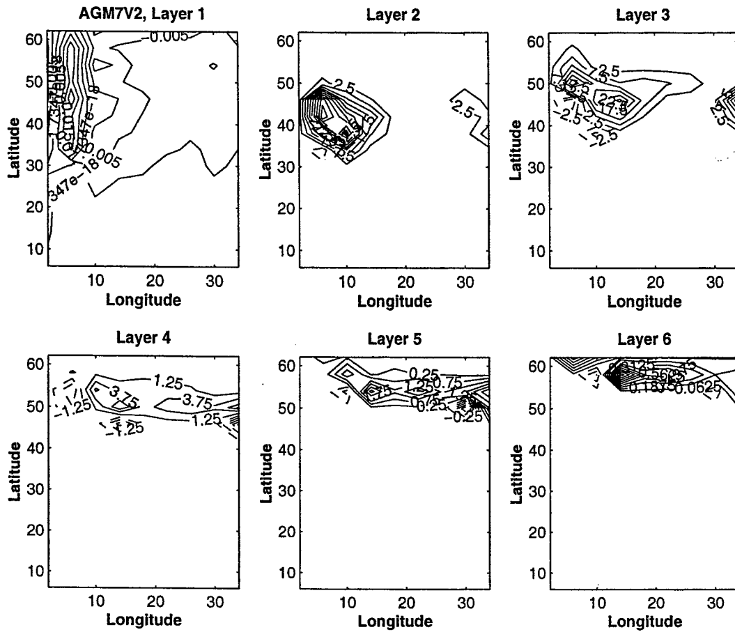
Figure 6-24: Flux divergence. Gent-McWilliams scheme. Experiment AGM7V2 ( K_{GM} = 10[M^2 \cdot \text{sec}^{-1}] , K_{Tw} = 0.3 \cdot 10^{-4}[M^2 \cdot \text{sec}^{-1}] ). Layers 1 to 6. Variable C.I. in 10^{-8} [^{\circ}\text{C} \cdot \text{sec}^{-1}] units. Divergence for Layer 1 < 10^{-10} [^{\circ}\text{C} \cdot \text{sec}^{-1}] .
