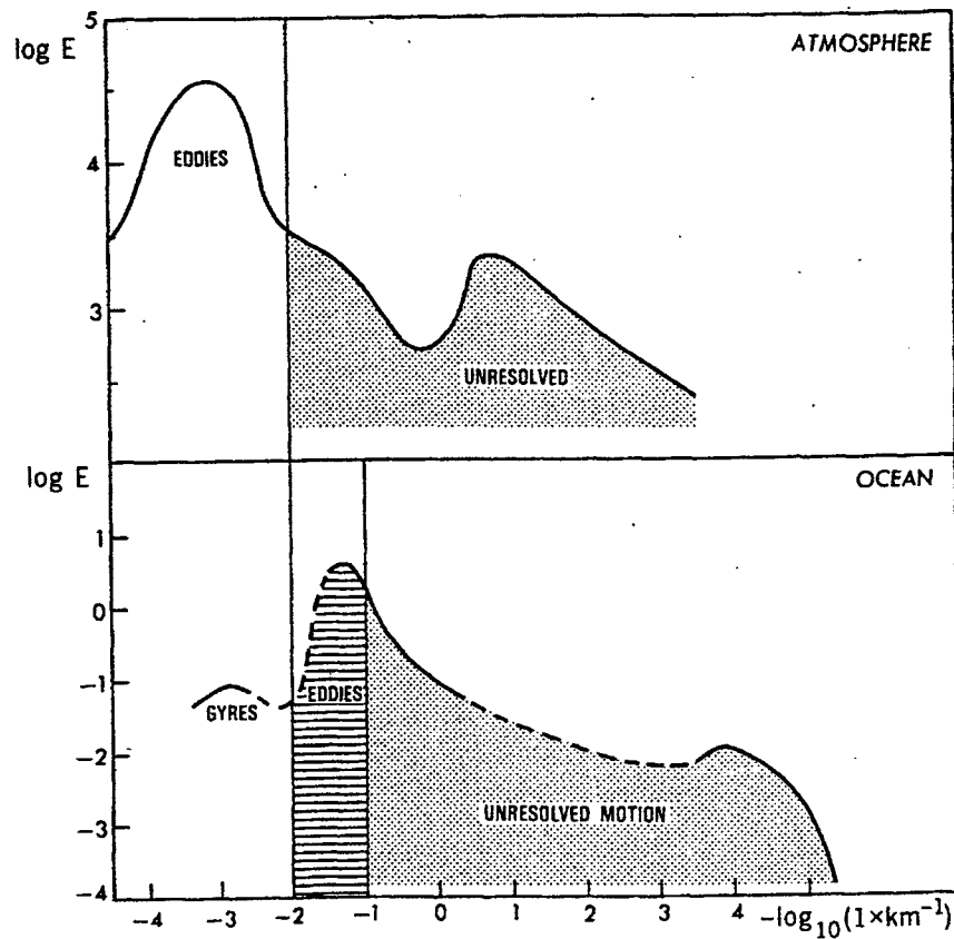
Figure 1-2: Kinetic energy spectrum, [M^2 \cdot \text{sec}^{-1}] , as a function of horizontal wave number, [\text{cycles}/KM] , for the atmosphere and the oceans. Adopted from Woods, 1985 [61].
