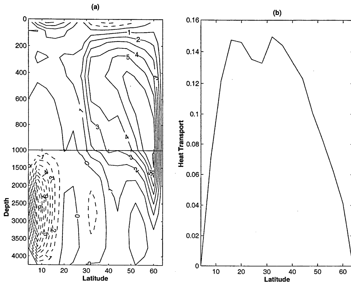
Figure 3-5: Transport properties of the reference simulation: (a) meridional overturning transport, [Sv] , stretched upper 1000M; (b) total Northward heat flux, [PW] .
