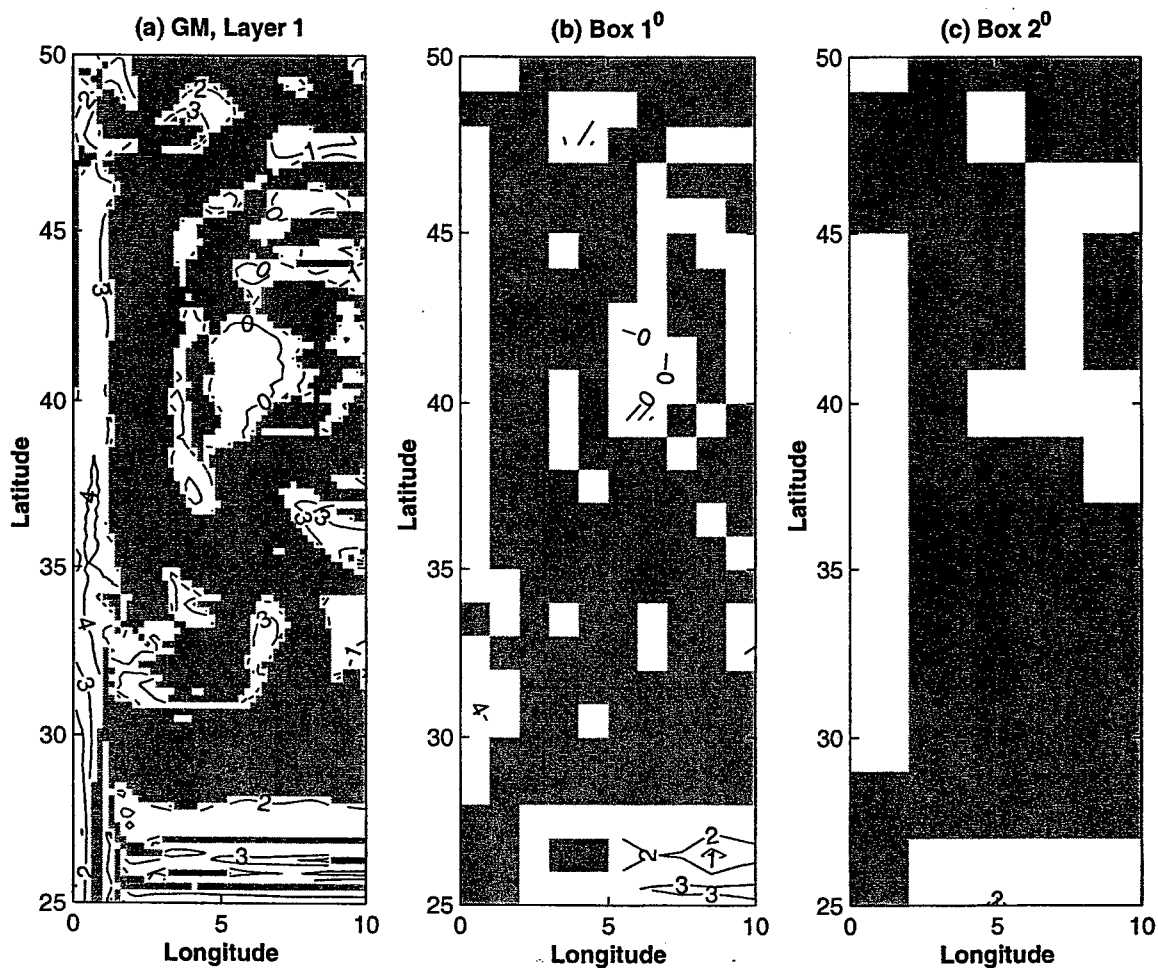
Figure 5-26: Test of the GM parameterization scheme. Layer 1. White areas: ratio_{GM} > 0 . Gray areas: ratio_{GM} \leq 0 . Contours value is \log_{10} of ratio_{GM} , [M^2 \cdot \text{sec}^{-1}] . (a) Fine resolution. Averaged over (b) 1^\circ \times 1^\circ and (c) 2^\circ \times 2^\circ .
