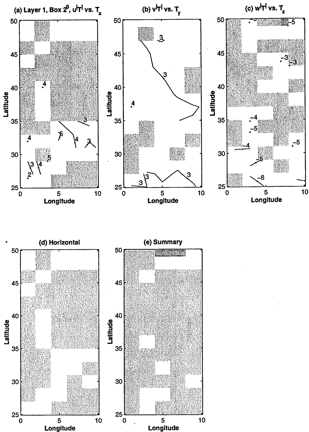
Figure 5-15: Test of the Fickian diffusivity on the 2^\circ \times 2^\circ grid. Layer 1. (a) K_{Tu} , (b) K_{Tv} , (c) K_{Tw} , (d) horizontal test, (e) summary of the test. White areas identify the positive diffusivity coefficients. Contour values are \log_{10} of the coefficients, [M^2 \cdot \text{sec}^{-1}] .
