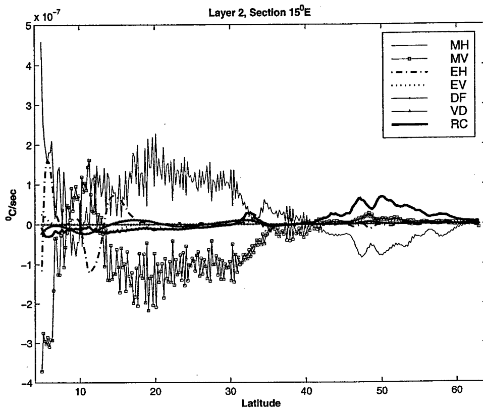
Figure 4-12: Balances in the temperature equation. Layer 2. Section at 15°E. MH - horizontal divergence of time-mean heat flux, MV - vertical derivative of time-mean flux, EH - horizontal divergence of eddy heat flux, EV - vertical derivative of eddy heat flux, DF - restoring diabatic forcing, VD - vertical diffusion, RC - residual implied convection.
