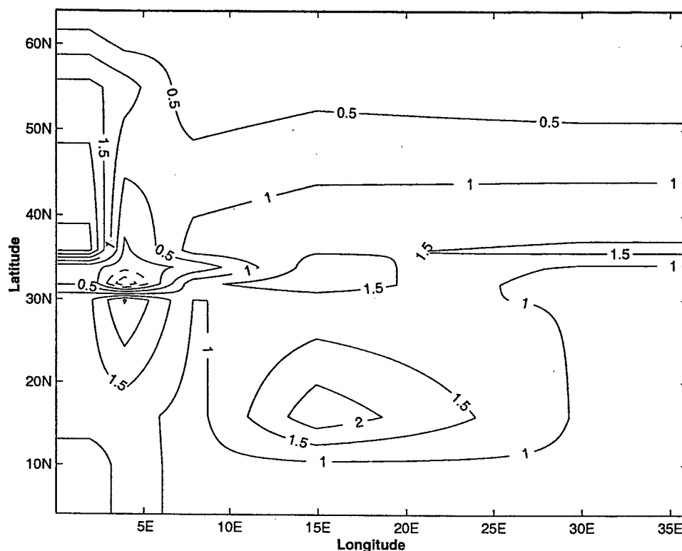
Figure 4-3: Contribution to the temperature balance of the local time-drift. Estimation from the time series, 10^{-9} [^{\circ}\text{C} \cdot \text{sec}^{-1}] for layer 5.
