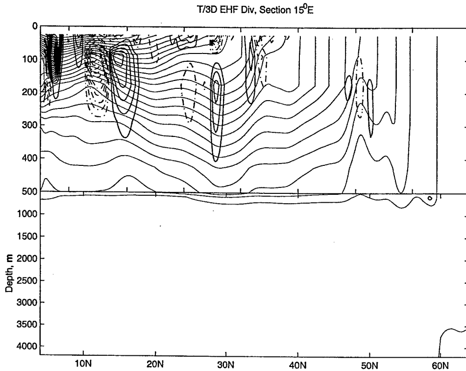
Figure 4-20: 3D divergence of the eddy heat flux, C.I. 10^{-8} [^{\circ}\text{C} \cdot \text{sec}^{-1}] , and isotherms of time-mean temperature, C.I. 1 [^{\circ}\text{C}] . Section at 15^{\circ}\text{E} .
