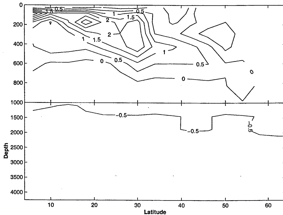
Figure 3-12: Zonally averaged temperature difference, [ ^{\circ}\text{C} ], between the reference experiment and the initial state of the reference fine resolution experiment, stretched upper 1000M.
