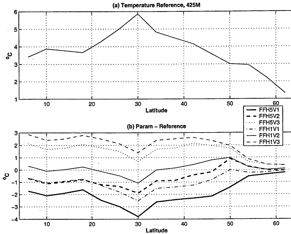
Figure 6-3: Zonally averaged temperature, section at 425M, [°C]. Fickian Diffusivity. (a) Reference experiment. (b) Parameterization experiments minus Reference. Labels identify experiments.
