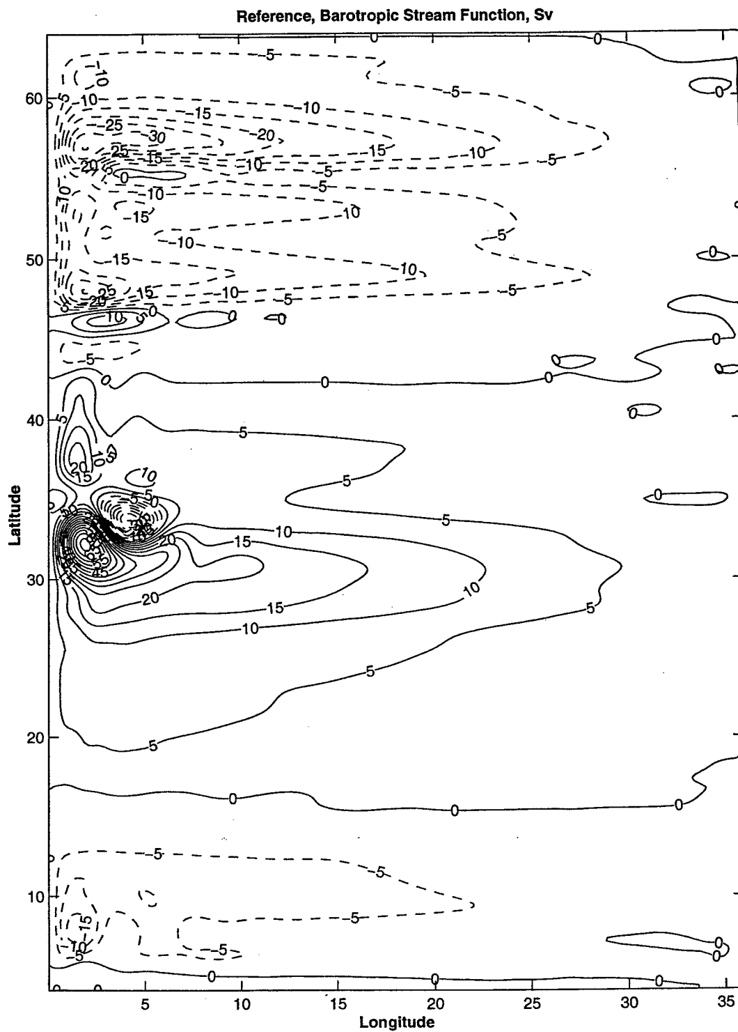
Figure 2-11: Barotropic transport, [Sv] in the reference experiment averaged over 55 years.
