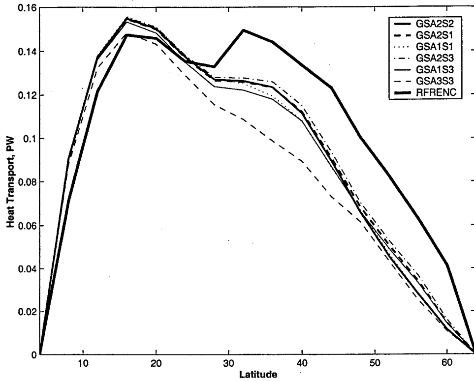
Figure 6-13: Total heat transport, [PW]. Green-Stone scheme. Labels identify experiments. RFRENC is the reference experiment.
