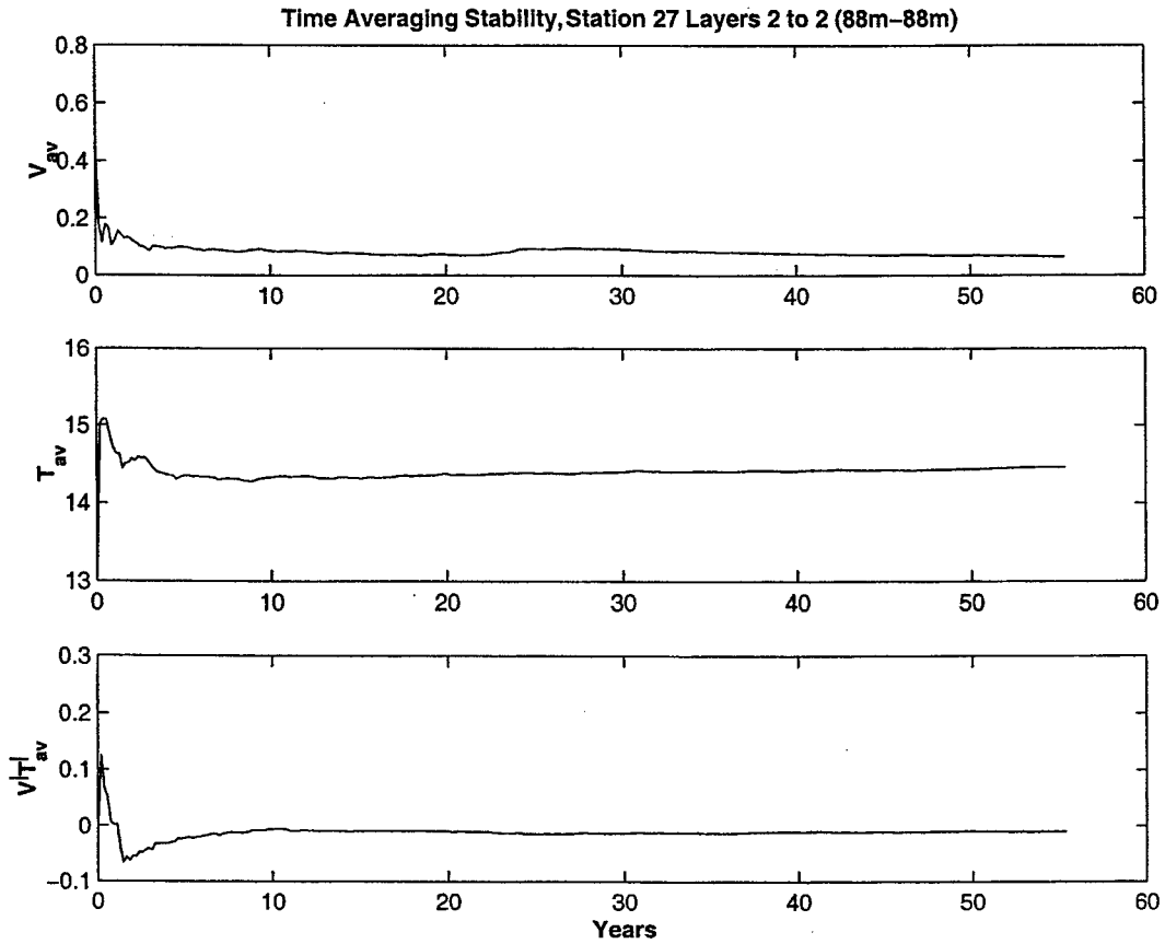
Figure 2-9: Stability of the time average quantities: upper plot: v , meridional velocity; middle plot: T , temperature; lower plot: v'T' , meridional heat flux. Station 27. Layer 2.
