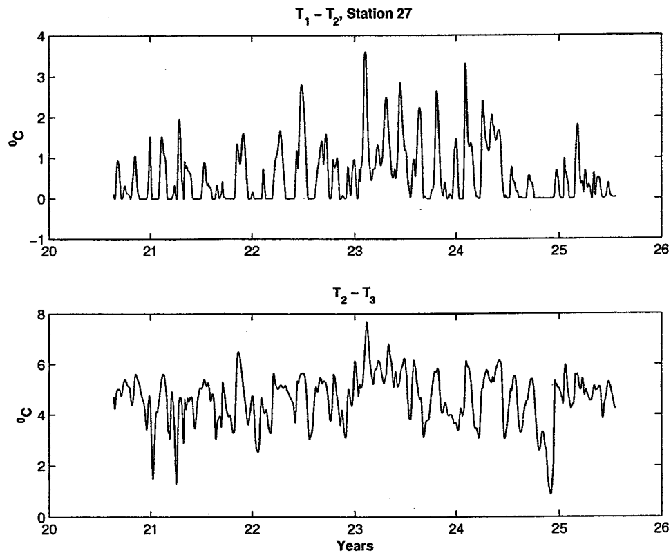
Figure 4-6: Upper layers convection. Station 27. Difference in temperature [ ^{\circ}\text{C} ] for layers 1-2 (25M-87.5M) upper panel, 2-3 (87.5M-175M) lower panel.
