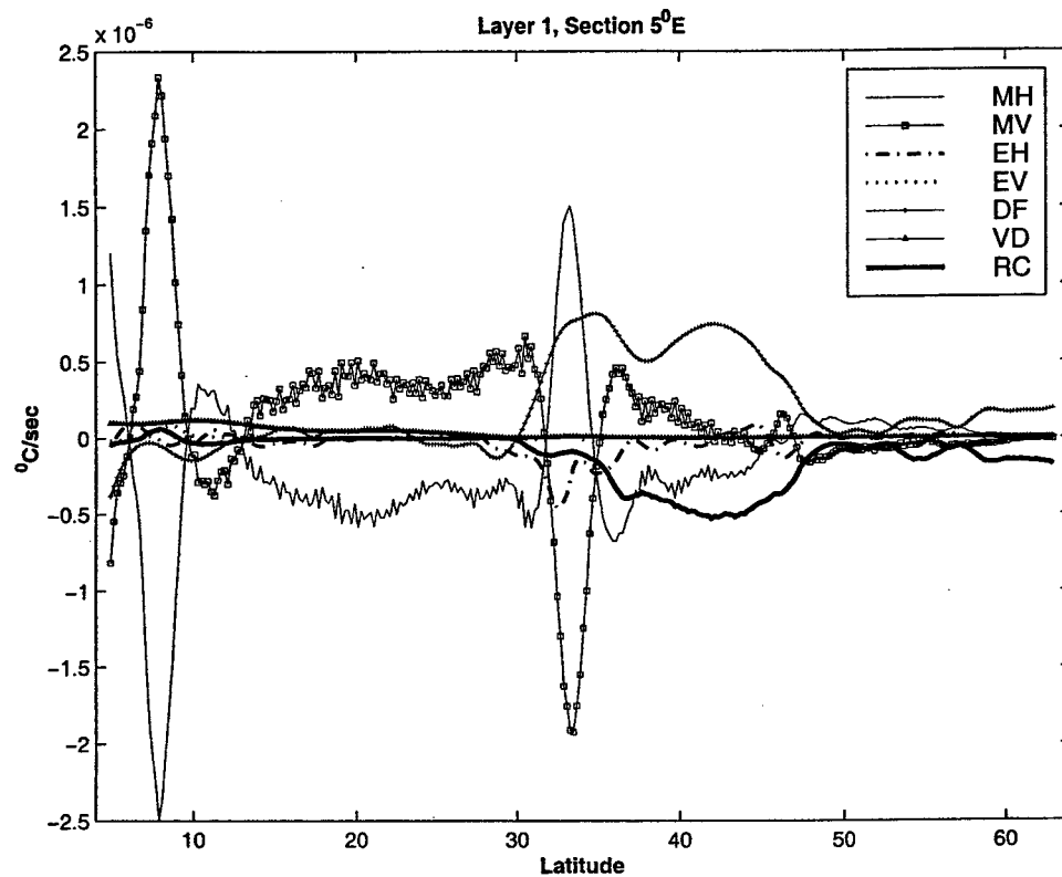
Figure 4-13: Balances in the temperature equation. Layer 1. Section at 5°E. MH - horizontal divergence of time-mean heat flux, MV - vertical derivative of time-mean flux, EH - horizontal divergence of eddy heat flux, EV - vertical derivative of eddy heat flux, DF - restoring diabatic forcing, VD - vertical diffusion, RC - residual implied convection.
