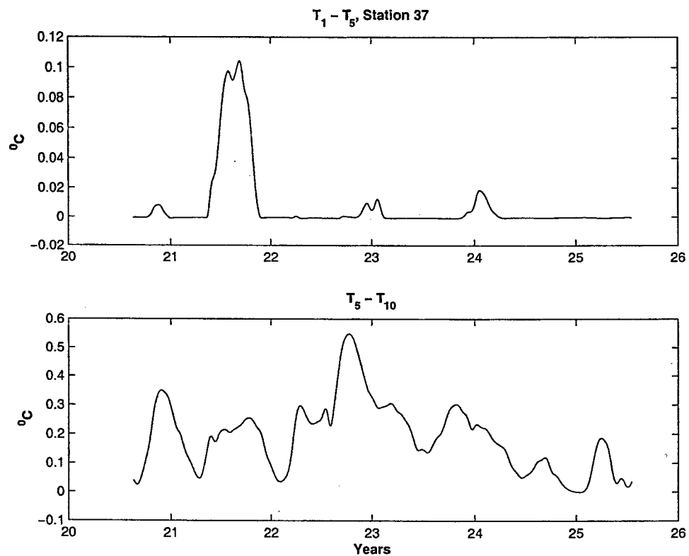
Figure 4-5: Convective events. Station 37. Northern part of the domain. Difference in temperature [ ^{\circ}C ] for layers 1-5 (25M-425M) upper panel, 5-10 (425M-1885M) lower panel.
