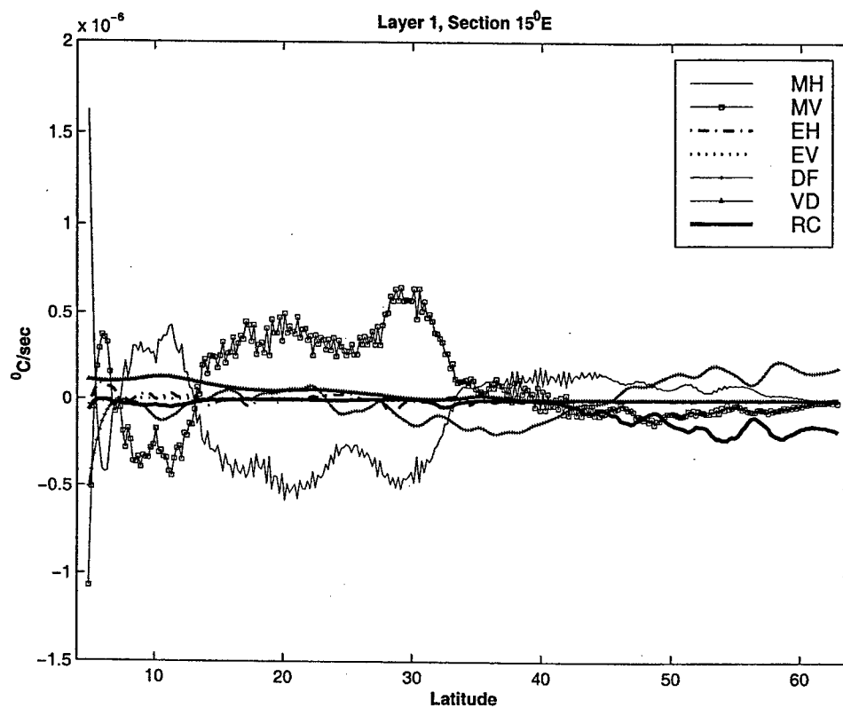
Figure 4-14: Balances in the temperature equation. Layer 1. Section at 15^{\circ}E . MH - horizontal divergence of time-mean heat flux, MV - vertical derivative of time-mean flux, EH - horizontal divergence of the eddy heat flux, EV - vertical derivative of the eddy heat flux, DF - restoring diabatic forcing, VD - vertical diffusion, RC - residual implied convection.
