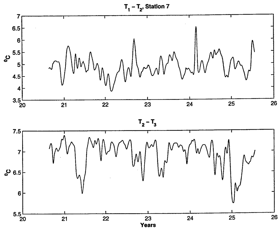
Figure 4-7: Stable stratification during the whole length of the simulation. Station 7. Temperature difference, [ ^{\circ}C ], for layers 1-2 (25M-87.5M) upper panel, 2-3 (87.5M-175M) lower panel.
