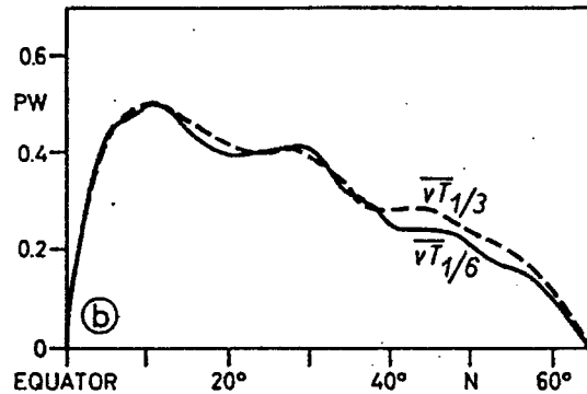
Figure 3-7: Total northward heat transport in the simulations by Cox, 1985 [13] (dashed line, 1/3^\circ resolution) and Böning and Budich, 1992 [4] (solid line, 1/6^\circ resolution). Adopted from Böning and Budich, 1992 [4].
