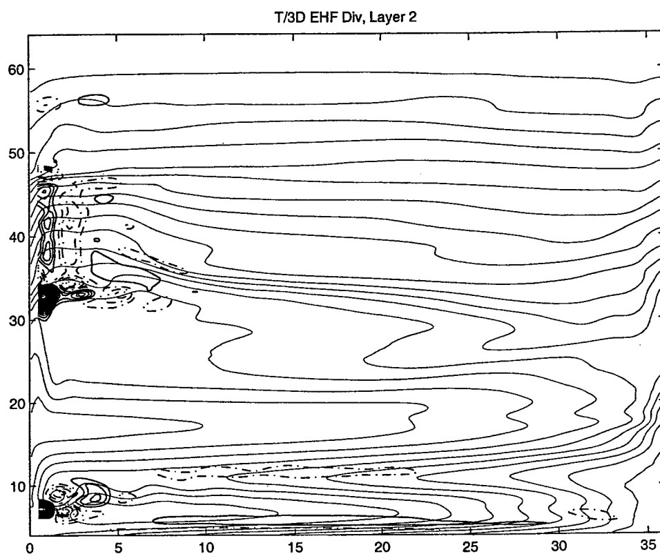
Figure 4-17: 3D divergence of the eddy heat flux, C.I. 10^{-7} [^{\circ}C \cdot \text{sec}^{-1}] , and isotherms of time-mean temperature, C.I. 1 [^{\circ}C] . Layer 2.
