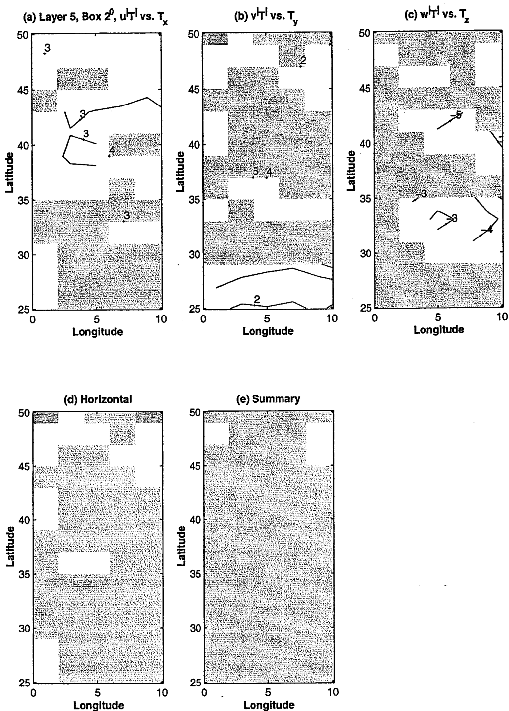
Figure 5-17: Test of the Fickian diffusivity on the 2^\circ \times 2^\circ grid. Layer 5. (a) K_{Tu} , (b) K_{Tv} , (c) K_{Tw} , (d) horizontal test, (e) summary of the test. White areas identify the positive diffusivity coefficients. Contour values are \log_{10} of the coefficients, [M^2 \cdot \text{sec}^{-1}] .
