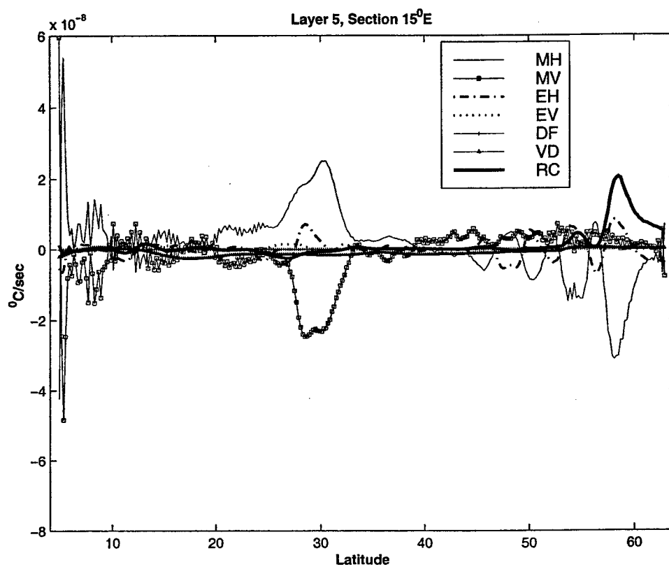
Figure 4-16: Balances in the temperature equation. Layer 5. Section at 15^{\circ}E . MH - horizontal divergence of time-mean heat flux, MV - vertical derivative of time-mean flux, EH - horizontal divergence of the eddy heat flux, EV - vertical derivative of the eddy heat flux, DF - restoring diabatic forcing, VD - vertical diffusion, RC - residual implied convection.
