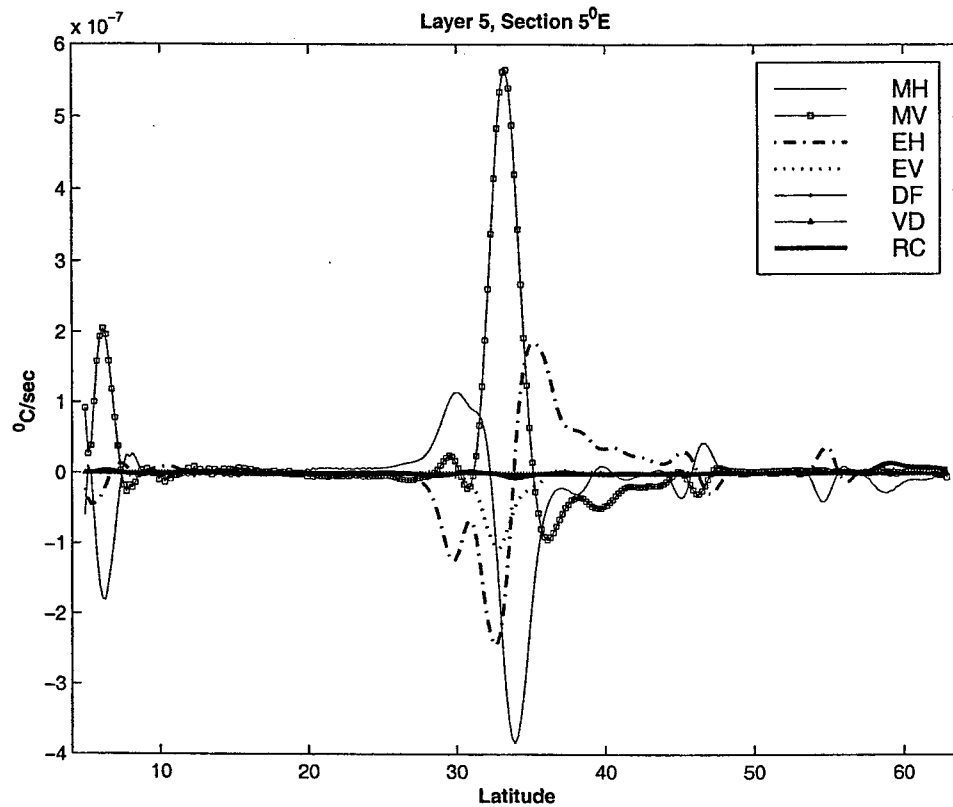
Figure 4-15: Balances in the temperature equation. Layer 5. Section at 5°E. MH - horizontal divergence of time-mean heat flux, MV - vertical derivative of time-mean flux, EH - horizontal divergence of the eddy heat flux, EV - vertical derivative of the eddy heat flux, DF - restoring diabatic forcing, VD - vertical diffusion, RC - residual implied convection.
