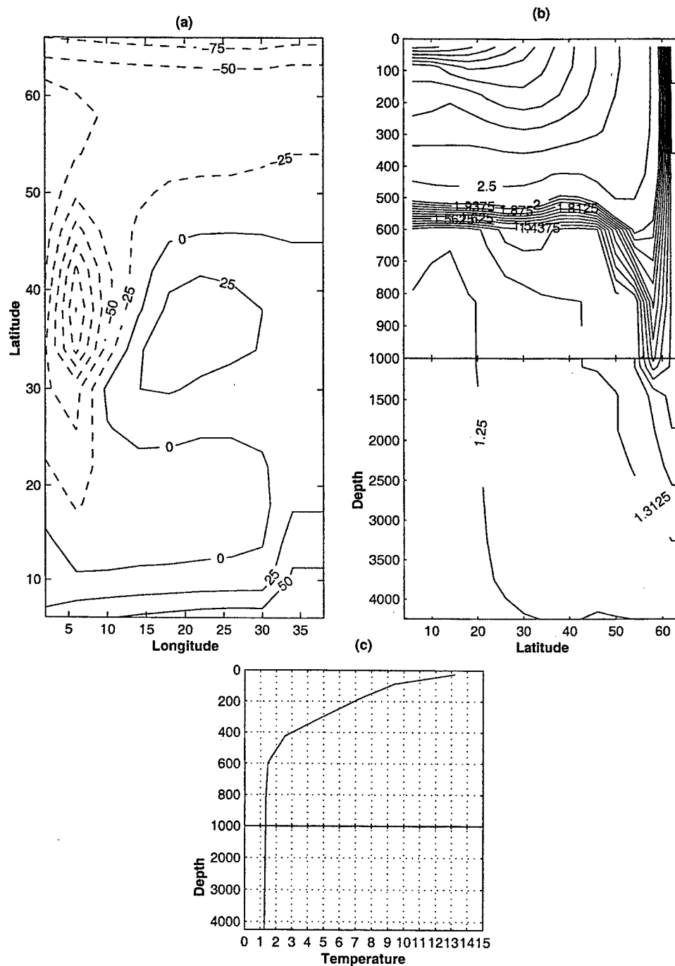
Figure 3-10: Thermal structure of the coarse resolution experiment: (a) surface heat flux, [W \cdot M^{-2}] ; (b) zonally averaged temperature, [^{\circ}C] , stretched upper 1000M, variable contour intervals of 0.0625^{\circ}C between 1^{\circ}C and 2^{\circ}C , 0.25^{\circ}C between 2^{\circ}C and 3^{\circ}C , 2.5^{\circ}C between 3^{\circ}C and 25^{\circ}C ; (c) horizontally averaged temperature, [^{\circ}C] , as a function of depth, stretched upper 1000M.
