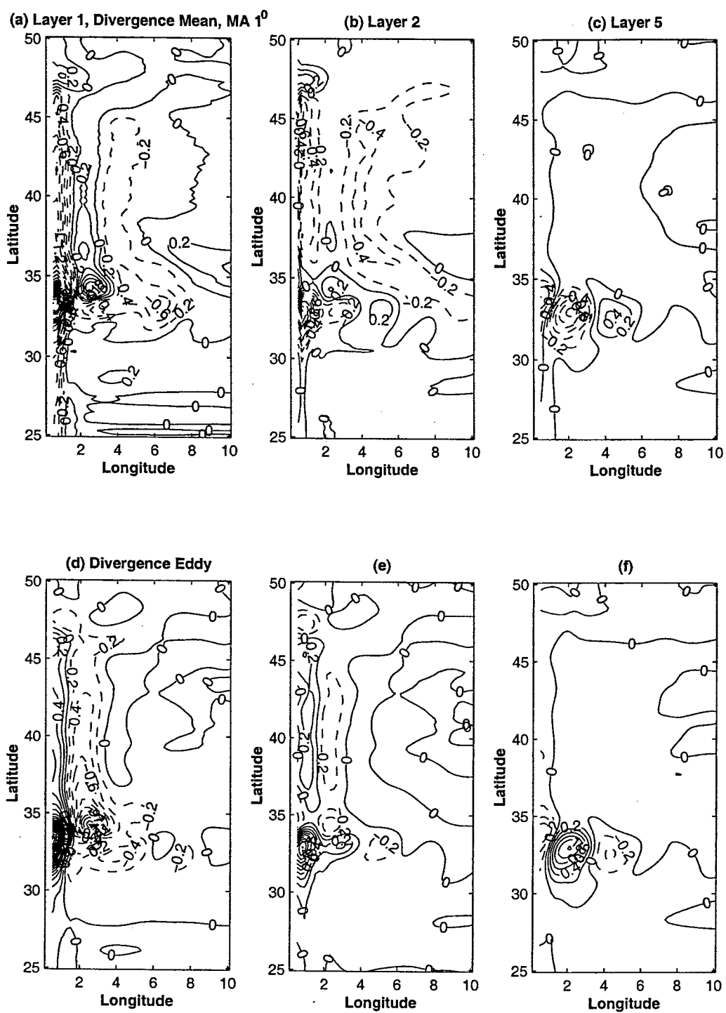
Figure 4-21: Three dimensional divergencies of the time mean (upper row) and eddy (lower row) heat fluxes. C.I. 0.2 \cdot 10^{-6} [^{\circ}C \cdot sec^{-1}] . Layer 1 (a,d), Layer 2 (b,e), Layer 5 (c,f).
