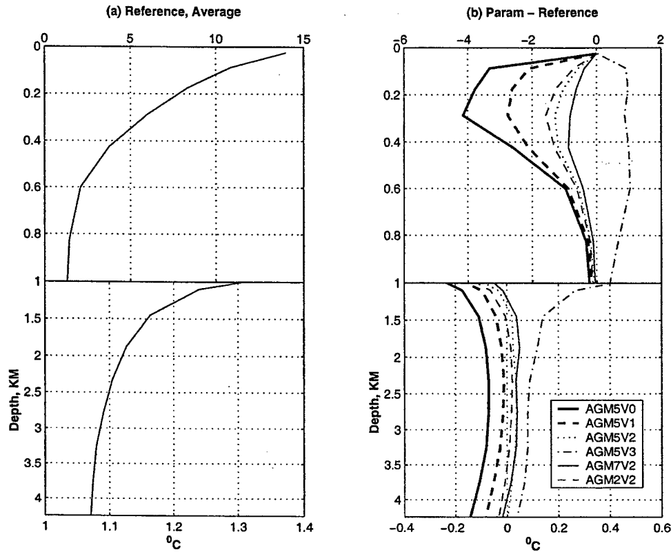
Figure 6-19: Horizontally averaged temperature, [ ^{\circ}\text{C} ]. Gent-McWilliams scheme. (a) Reference experiment. (b) Parameterization experiments minus Reference. Stretched upper 1000M. Labels identify experiments.
