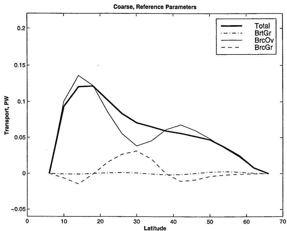
Figure 3-17: The decomposition of the total integrated northward heat transport ( Total ) of the coarse resolution experiment into heat transport by the barotropic gyre ( BrtGr ), baroclinic overturning ( BrcOv ) and baroclinic gyre ( BrcGr ) components, [PW].
