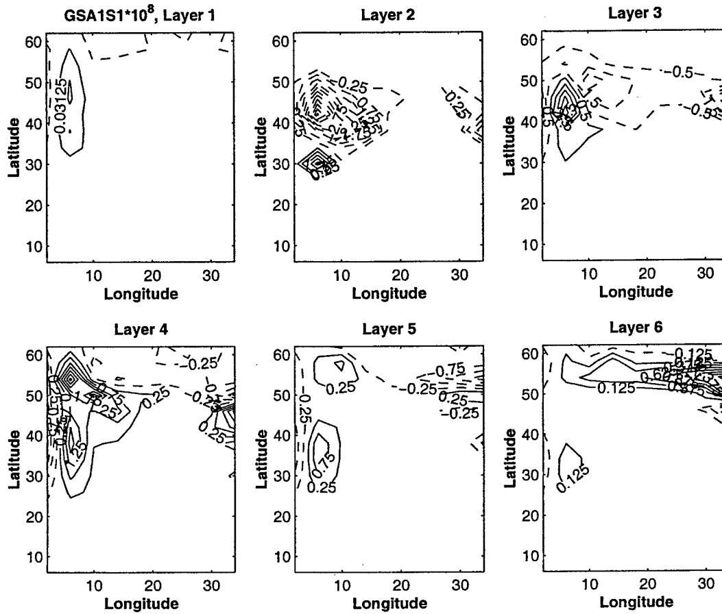
Figure 6-16: Flux divergence. Green-Stone scheme. Experiment GSA1S1 ( \alpha = 0.02 , \max(\hat{s}_{IS}) = 10^{-3} ). Layers 1 to 6. Variable C.I. in 10^{-8} [^{\circ}\text{C} \cdot \text{sec}^{-1}] units.
