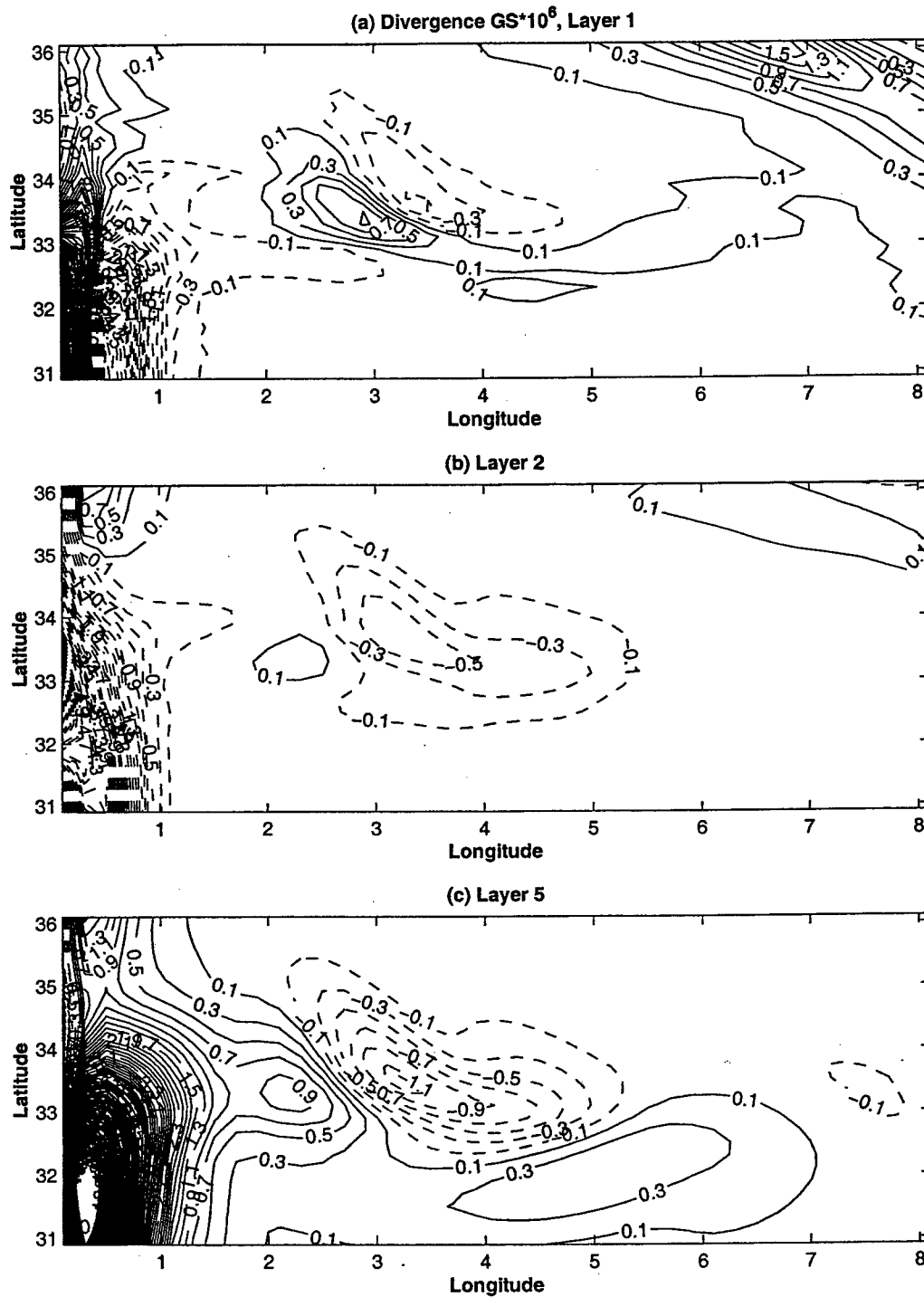
Figure 5-25: Divergence of the heat flux estimated with the GS parameterization scheme. C.I. 0.2 \cdot 10^{-6} [^{\circ}\text{C} \cdot \text{sec}^{-1}] . (a) Layer 1, (b) Layer 2, (c) Layer 5.
