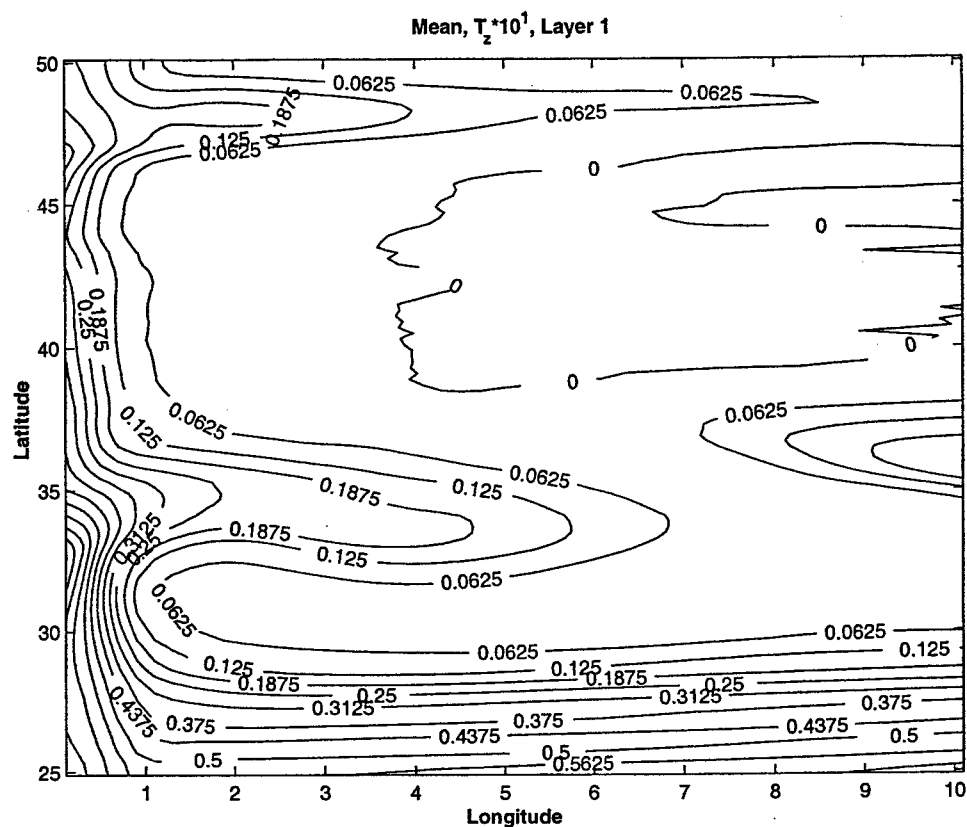
Figure 5-11: Distribution of \bar{T}_z , evaluated at the interface between the first and second layers, [ 10^{-1} C \cdot M^{-1} ].
