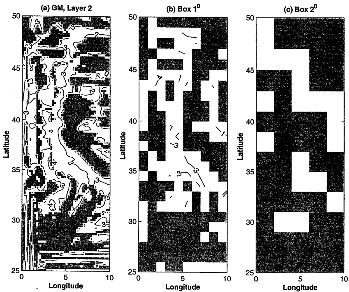
Figure 5-27: Test of the GM parameterization scheme. Layer 2. White areas: ratio_{GM} > 0 . Gray areas: ratio_{GM} \leq 0 . Contours value is \log_{10} of ratio_{GM} , [M^2 \cdot \text{sec}^{-1}] . (a) Fine resolution. Averaged over (b) 1^\circ \times 1^\circ and (c) 2^\circ \times 2^\circ .
