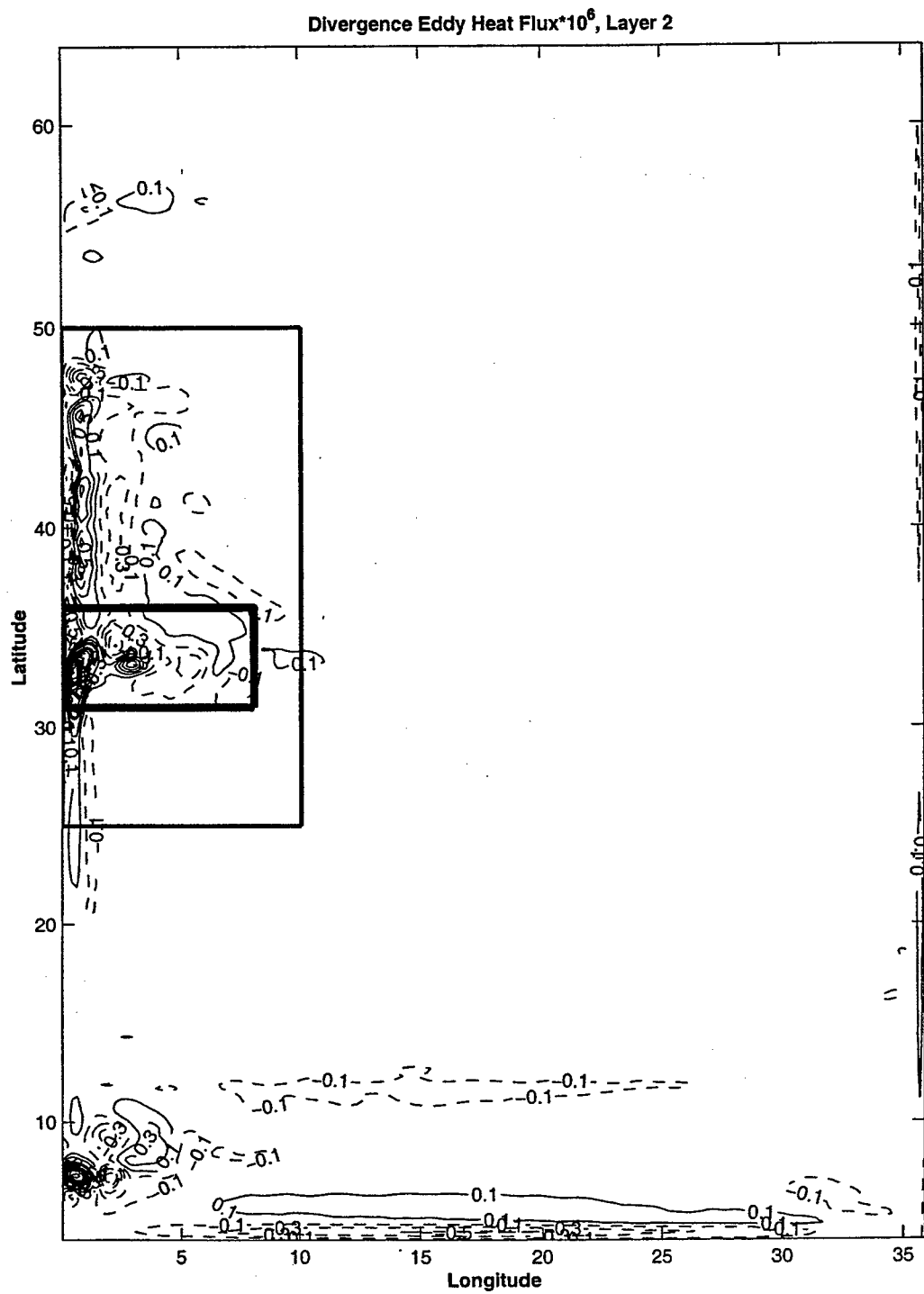
Figure 5-5: Divergence of the eddy heat flux. Layer 2. C.I. 0.2 \cdot 10^{-6} [^{\circ}\text{C} \cdot \text{sec}^{-1}] .
