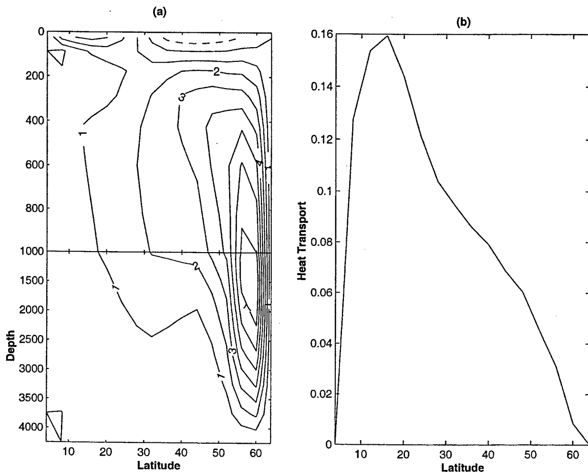
Figure 3-9: Transport properties of the initial state: (a) meridional overturning transport, [Sv] , stretched upper 1000M; (b) total Northward heat flux, [PW] .
