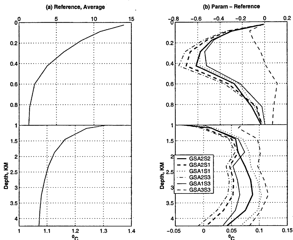
Figure 6-11: Horizontally averaged temperature, [\text{C}] . Green-Stone scheme. (a) Reference experiment. (b) Parameterization experiments minus Reference. Stretched upper 1000M. Labels identify experiments.
