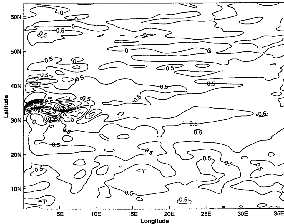
Figure 4-4: Contribution to the temperature balance of the local time-drift. Estimation from the temperature fields at iterations 1304580 and 3491712, 10^{-9} [^{\circ}\text{C} \cdot \text{sec}^{-1}] for layer 5.
