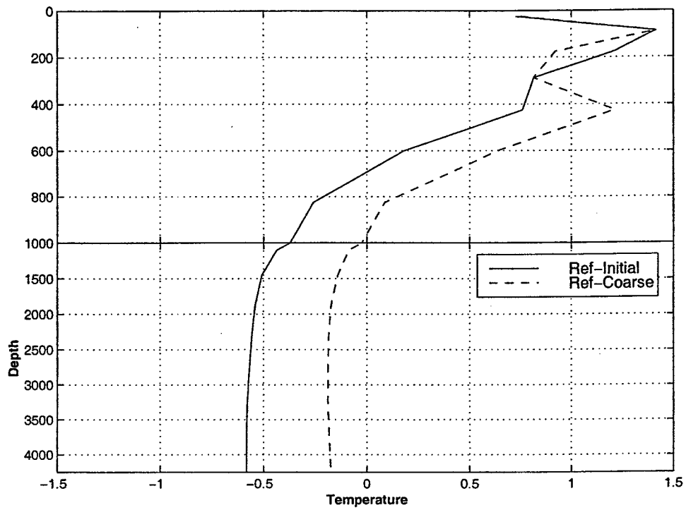
Figure 3-14: Horizontally averaged temperature difference, [^{\circ}\text{C}] , as a function of depth between the climatology and the initial state of the reference fine resolution simulation and the coarse resolution experiments, upper 1000M is stretched.
