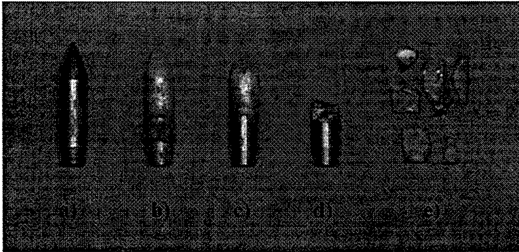
Figure 4. Typical Examples of Core Damage. From Left to Right: a) Pristine, b) Tip Eroded, c) Tip Fractured, d) Body Fractured, and e) Body Shattered.
