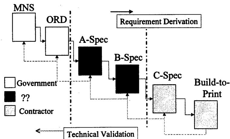
Figure 3. Systems Engineering Process
