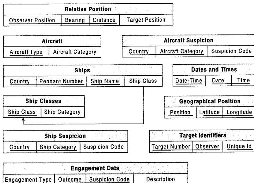
Figure D11: The relational schema for storing the predefined data.
