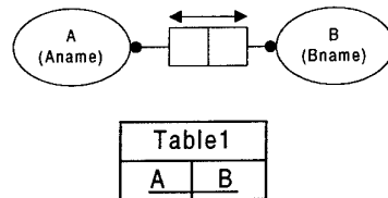
Figure C1: A fact type with a composite key.
