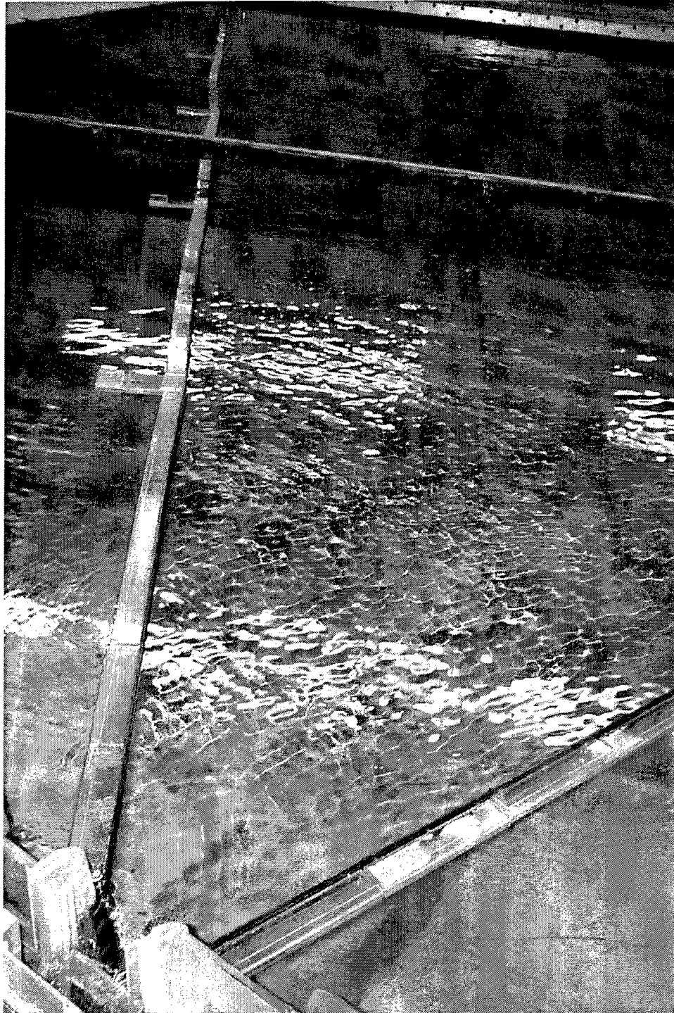
Figure 8. Original trash boom assembly installed in model
