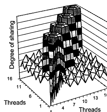
Figure 7: 16-thread FFT
