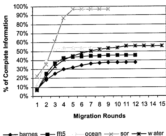
Figure 6: Passive information-gathering
