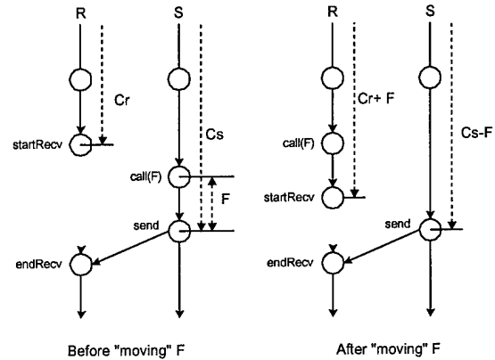
Figure 3: Computing procedure LBF - The PAG before and after moving the procedure F . The time for the procedure F is moved from the sending process (which is on the application's critical path) to the receiving one (which is not).
