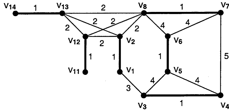
Figure 27: Graph \Gamma for the set of primitive line segments in Figure 26. Thick edges correspond to line segments. Thin edges signify other type of geometric relationship.
