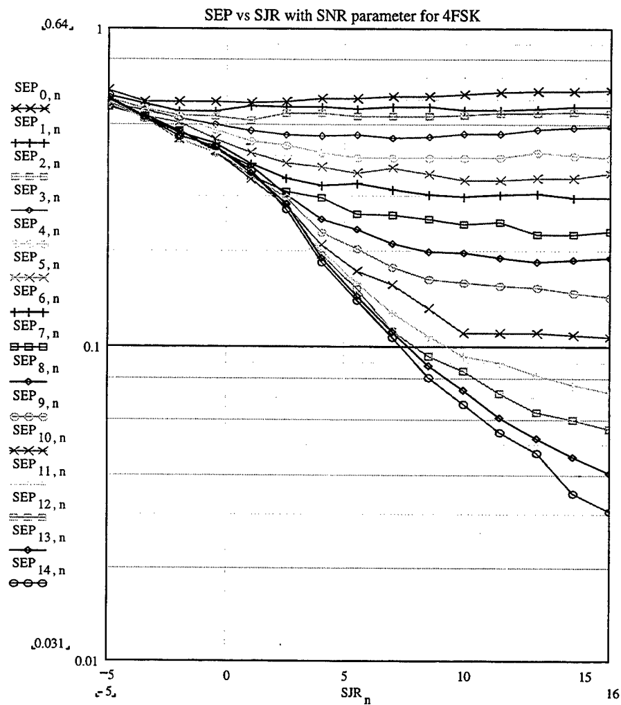
Figure 184. Simulation symbol error probability versus SJR with SNR as a parameter for non-coherent 4FSK, with Rician fading and R=1 for both MFSK signals (desirable and interfering).
