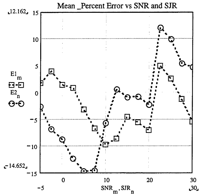
Figure 72. Mean percent difference as a function of SNR and SJR, respectively.
