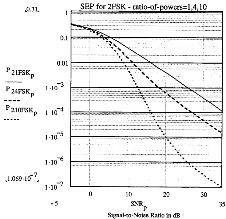
Figure 20. Probability of symbol error for coherent detection of 2FSK signals in Rician
