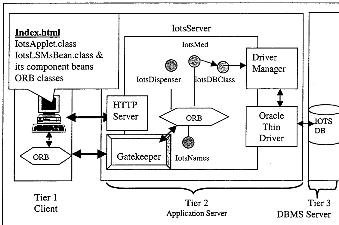
Figure 36. The IOTS Prototype Components
