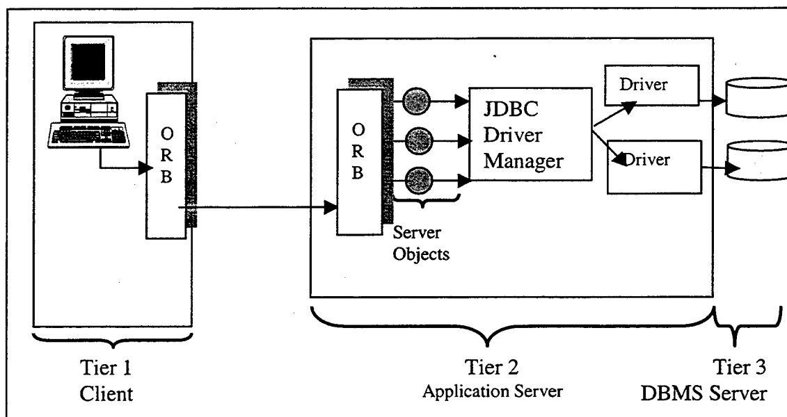
Figure 19. Three-tier (Orfali, 1998, 586)
