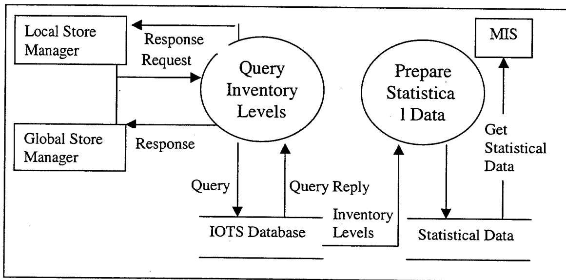
Figure 5. Placing Queries
