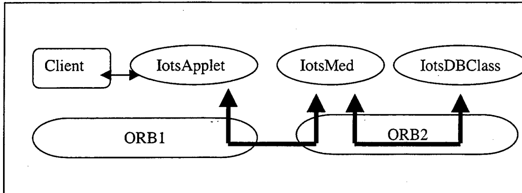
Figure 43. ORB-to-ORB Interoperability
