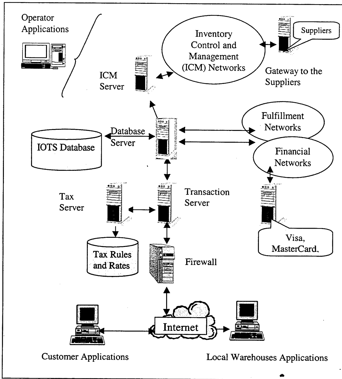
Figure 31. System Architecture
