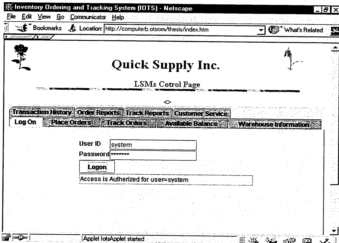
Figure 37. Logon Form
