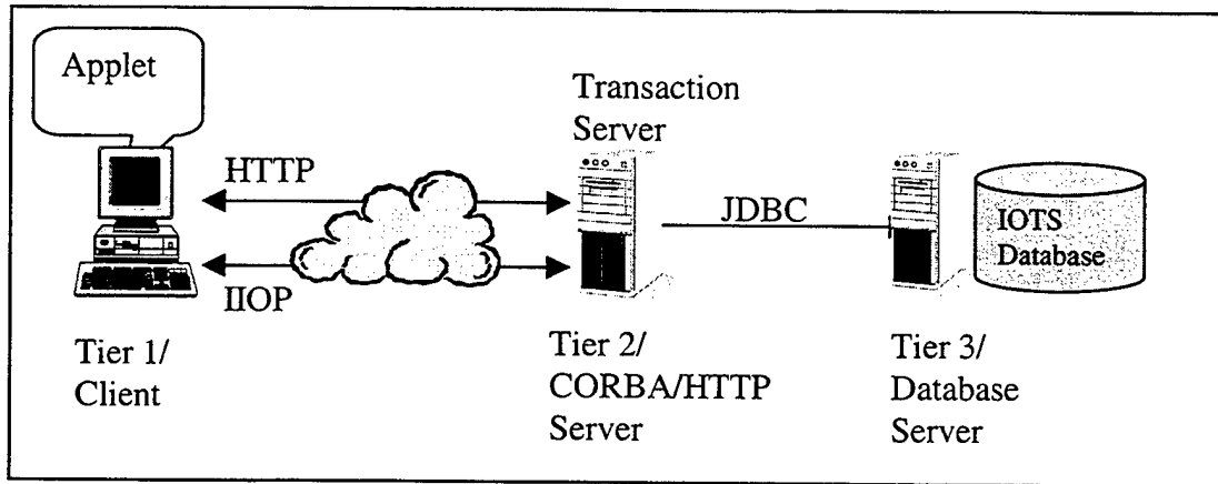
Figure 35. The IOTS in a Three-tiered Client/Server Architecture
