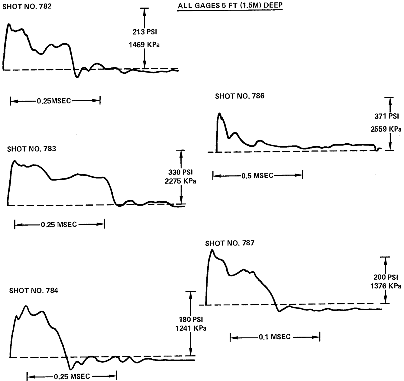
FIG. 2 DISTORTED PRESSURE WAVEFORMS.
