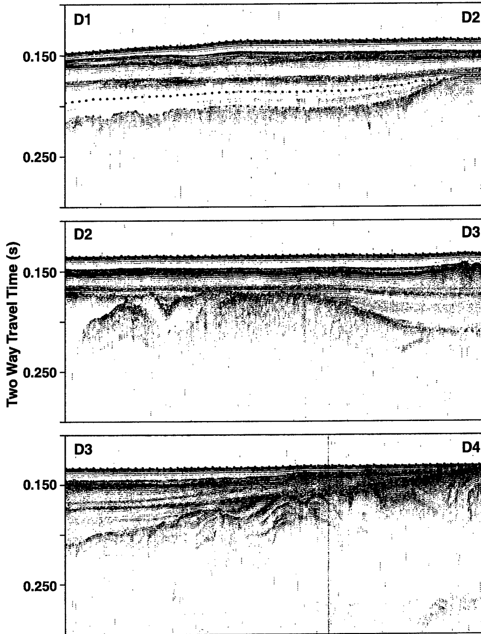
Figure 4 (D): Single channel seismic reflection profile segments from track boom04 (see figure 2 for location). Seismic Units 1, 2, 3, and 4 are bounded by the unconformities which are colour coded red (seabed), green, blue, magenta, and orange (acoustic basement) respectively. Note overlap of sequence boundaries to acoustic basement in D1-D2 and D3-D4. Clip set to 400.
