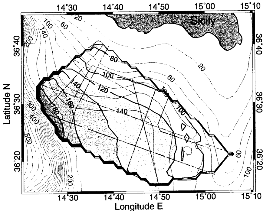
Figure 3: A comparison of bathymetry from the R/V Alliance echo sounder (black contours with gray shading) at positions along the seismic tracks (red) and DBDB-V (blue contours).
