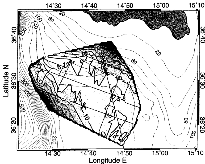
Figure 7: Isopach map of seismic Unit 1 in two way travel time (black contours in milliseconds with gray shading). Contours (in 20 m intervals) of DBDB-V bathymetry are in blue.
