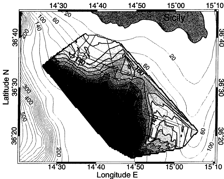
Figure 5: Depth to acoustic basement in two way travel time (black contours in milliseconds with gray shading). Contours (in 20 m intervals) of DBDB-V bathymetry are in blue.
