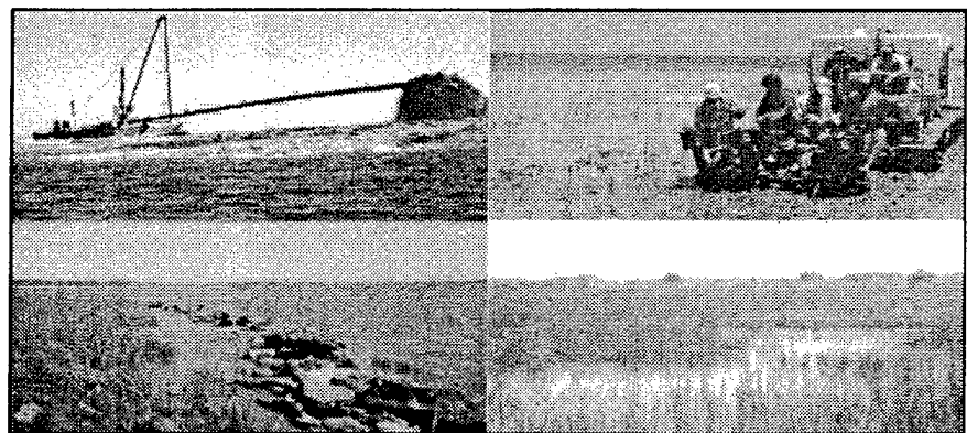
Figure 1. Marshes can be constructed by placing dredged material on shallow bay bottoms to build up elevations to an intertidal level, usually by pumping hydraulically dredged material to the marsh construction site (upper left). At sites exposed to high wind or wave energy, protective structures, such as riprap breakwaters (lower left), are built to protect dredged material. Vegetation can be actively planted (upper right), although some projects rely on natural recruitment. Within two to three growing seasons, dredged material marshes can appear similar to natural marshes (lower right). Photographs from U.S. Army Engineer Research and Development Center, Waterways Experiment Station.
