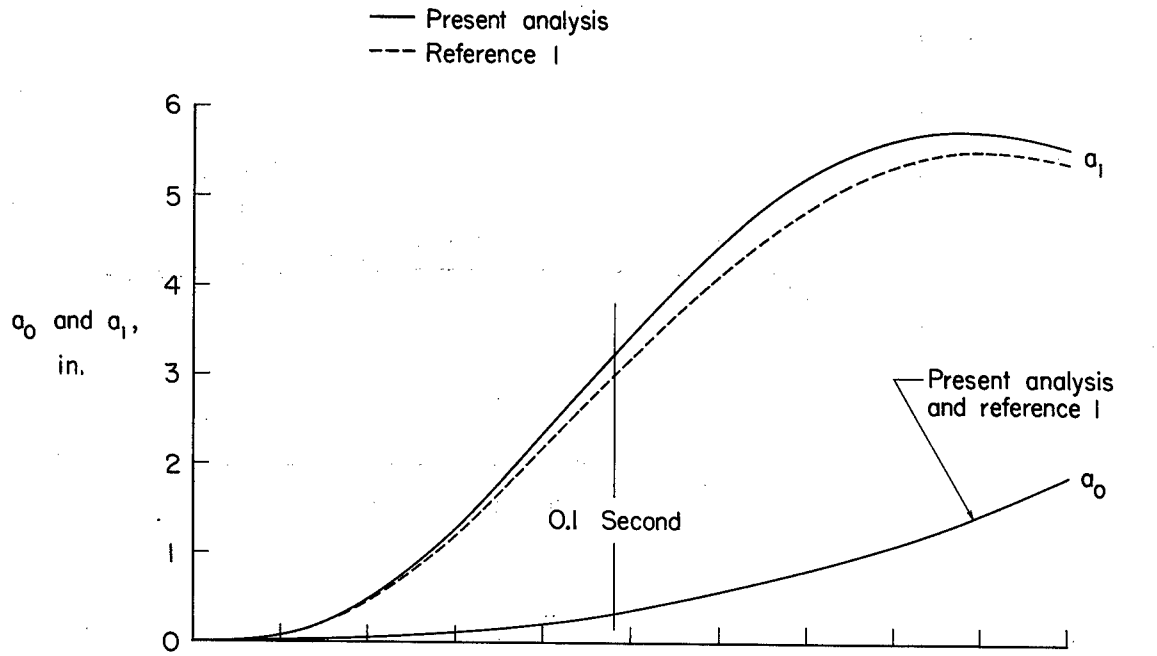
(a) Displacements.
