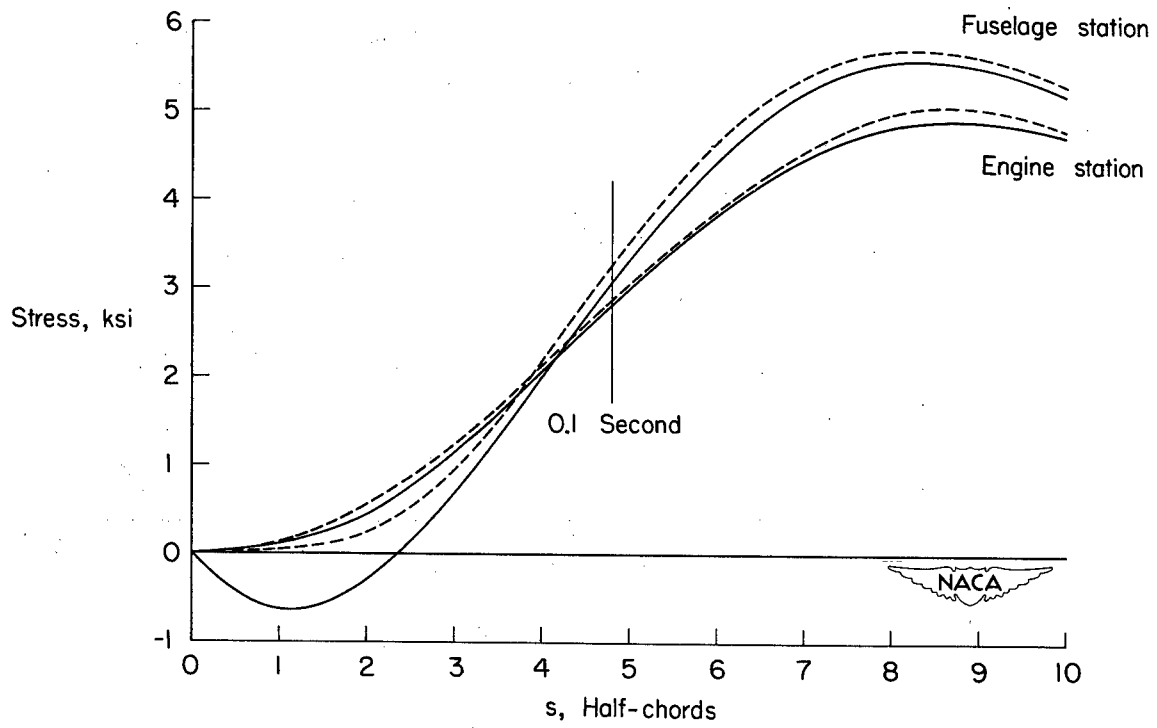
(b) Stresses.
