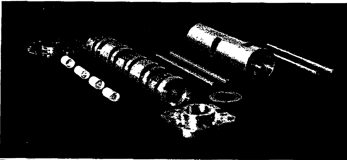
Fig. 3. Photograph of the disassembled components for the UCD TE_{0n} gyrokystron circuit. Clockwise from the upper left, the six groups are: 1) the dielectric rings to load the cavities and drift-tubes; 2) the cavities and drift-tubes; 3) two alignment posts; 4) the circuit enclosure; 5) two more alignment posts; and 6) the base for the circuit.
