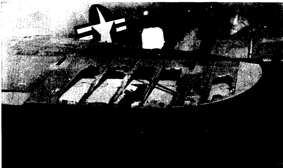
Figure 16.- Hail case 14. DC-3 airplane. Right elevator. (Time in hail unknown; TAS 170 mph.)
