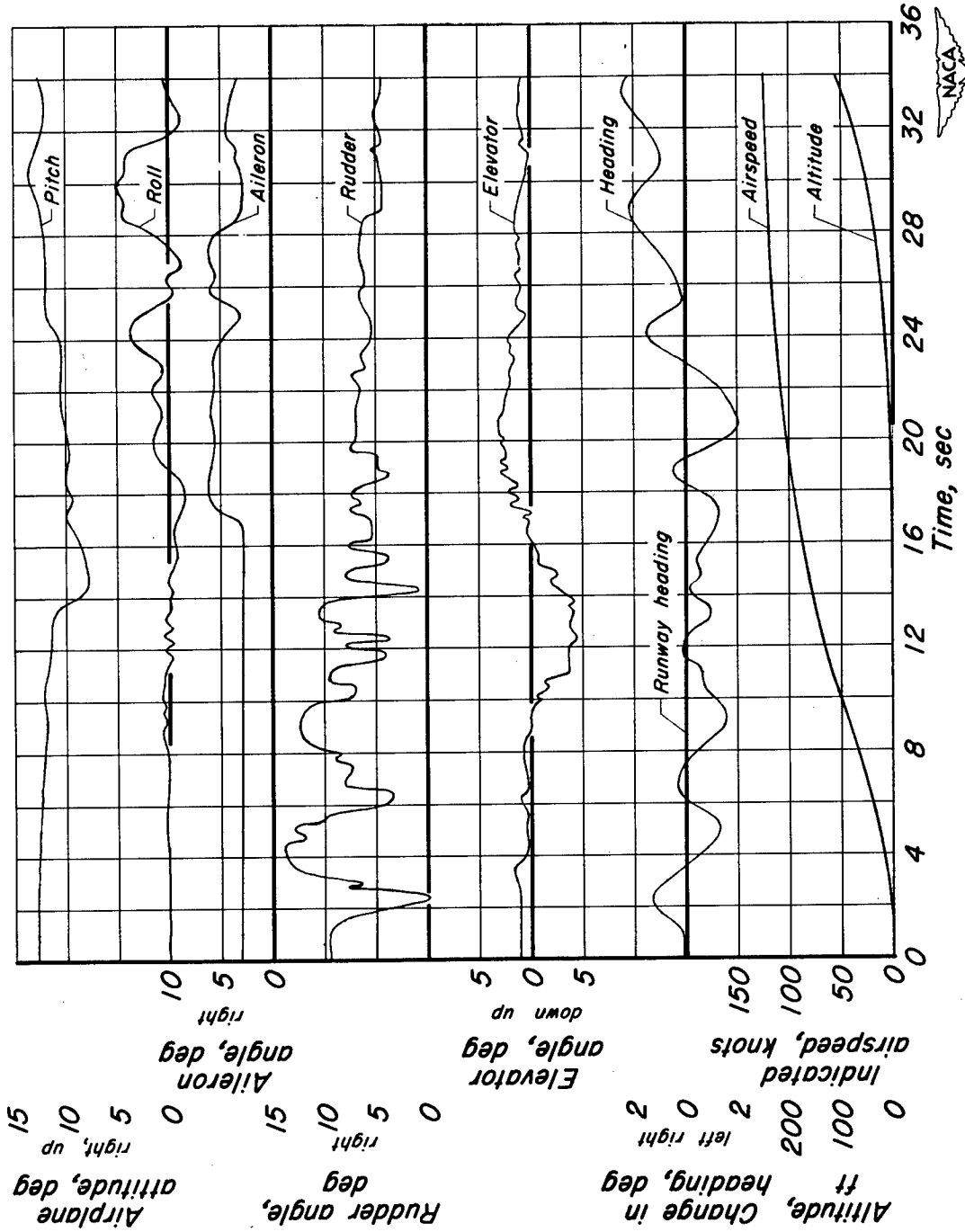
(c) Manually controlled, no cross wind, SB2C-5, drone # 83135. Figure 16. - Concluded.
