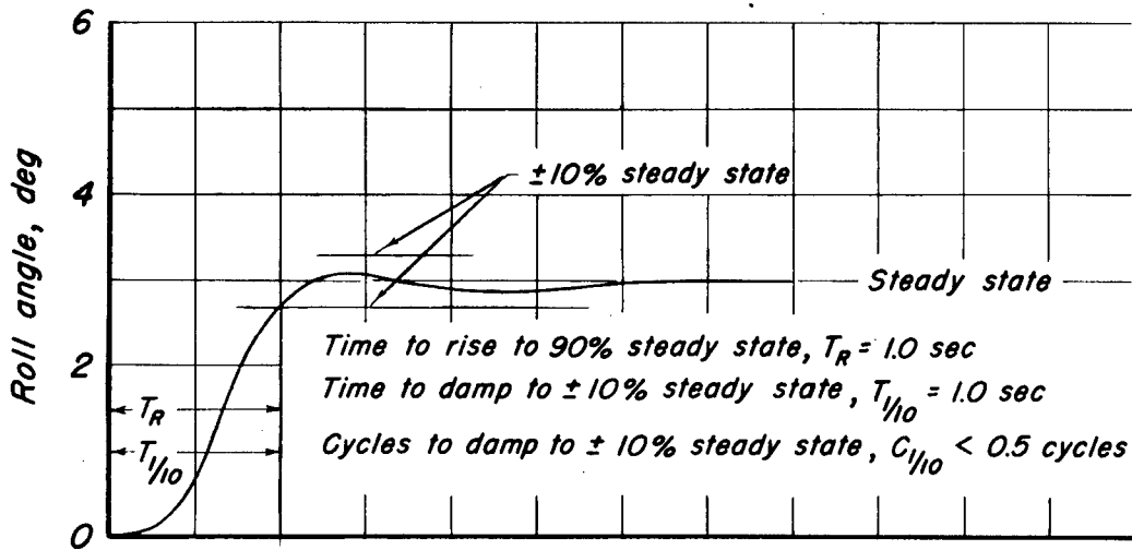
(a) Roll response to step input, rudder locked; follow-up sensitivity 45; rate sensitivity 30.
