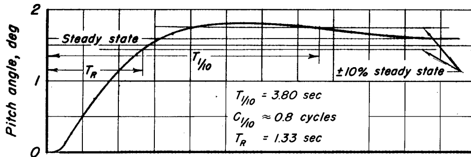
(a) Follow-up sensitivity 70.
