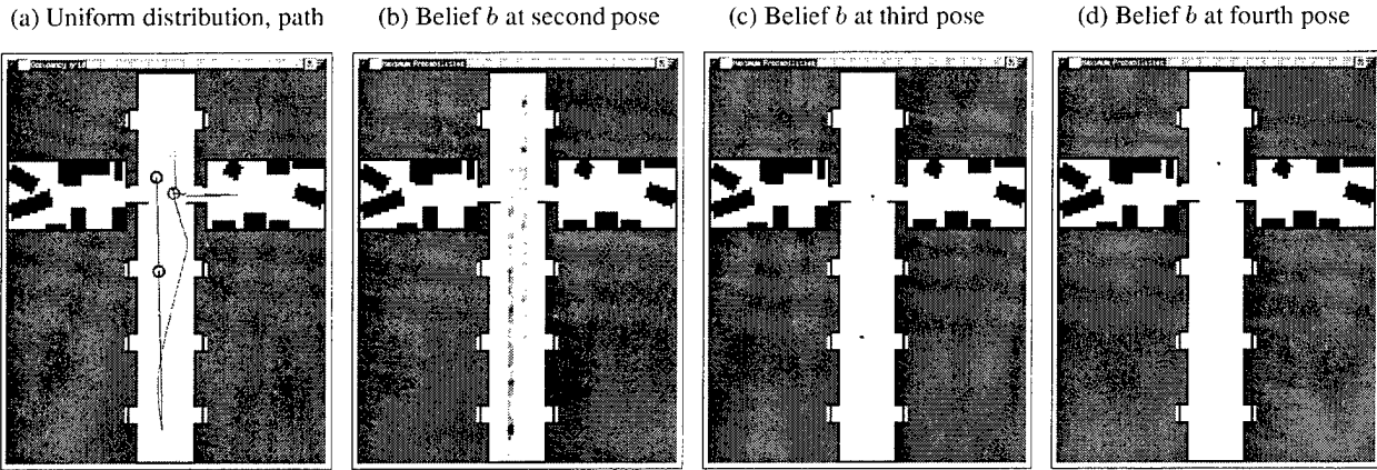
Figure 3: Example of grid-based Markov localization in a symmetric environment. (a) robot path, highlighting four robot poses, (b) to (d): belief b at 2nd, 3rd, and 4th pose, respectively.
