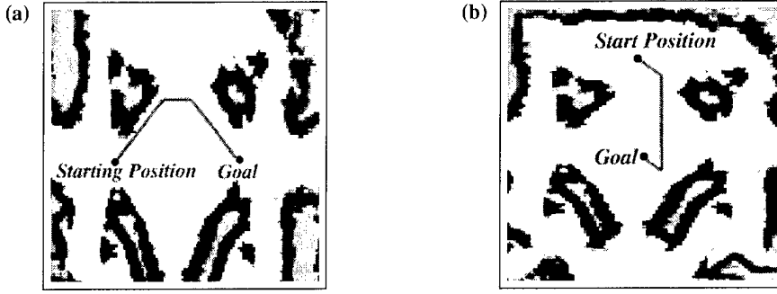
Figure 6: Coastal plans: the robot actively seeks the proximity of obstacles to improve its localization. The large open area in the center of this Smithsonian museum is approximately 20 meters wide and usually crowded with people.
