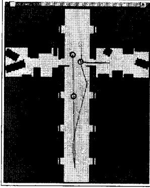
Figure 3: Example of grid-based Markov localization in a symmetric environment. (a) robot path, highlighting four robot poses, (b) to (d): belief at 2nd, 3rd, and 4th pose, respectively.
