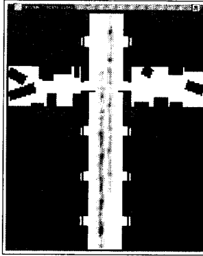
Figure 3: Example of grid-based Markov localization in a symmetric environment. (a) robot path, highlighting four robot poses, (b) to (d): belief at 2nd, 3rd, and 4th pose, respectively.
