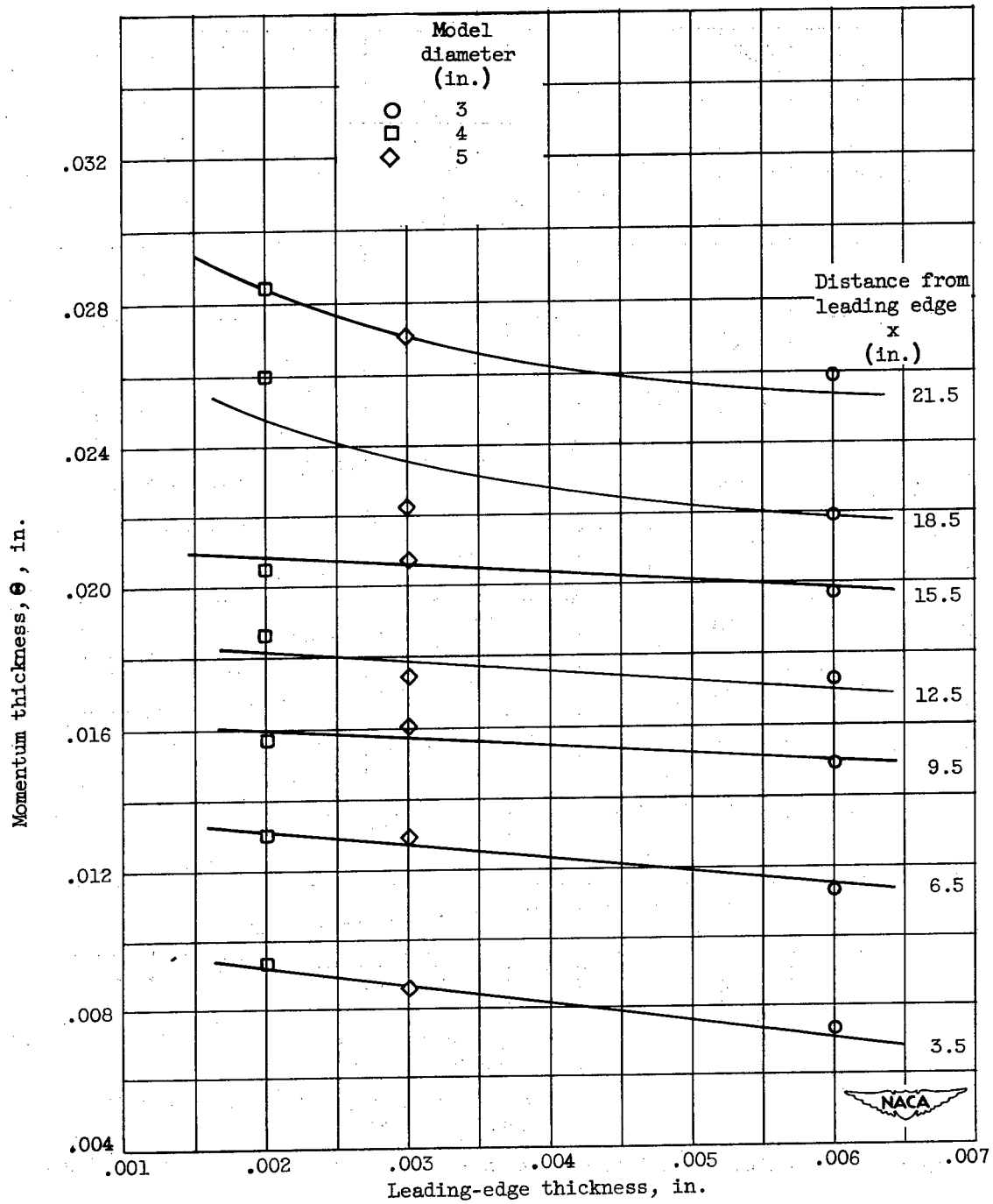
(c) Artificial transition, stagnation pressure of 12 pounds per square inch absolute.
