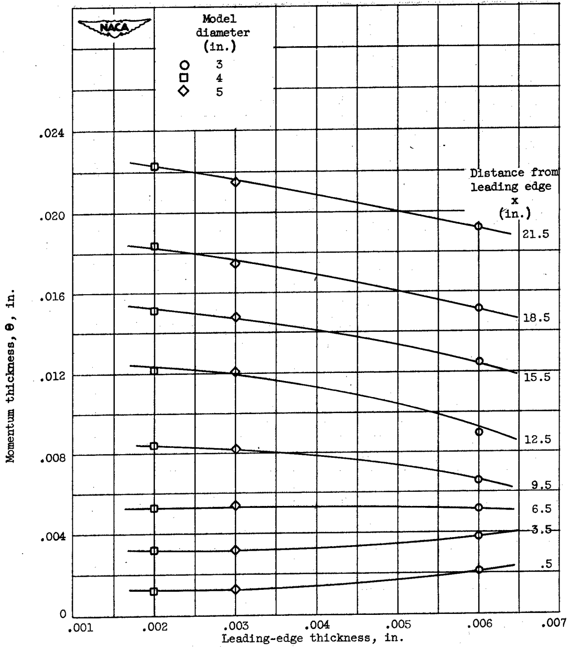
(a) Natural transition, stagnation pressure of 12 pounds per square inch absolute.
