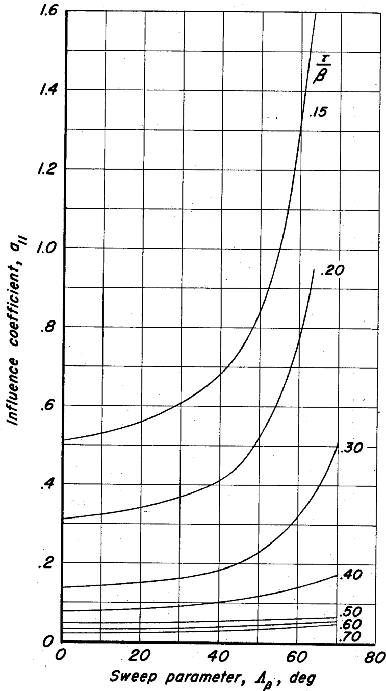
Figure 17.- Influence coefficients, a_{yn} , for symmetric span loading plotted as a function of the sweep parameter, \Delta_p , for various distances ahead of the wing quarter-chord line, \tau/\beta .
