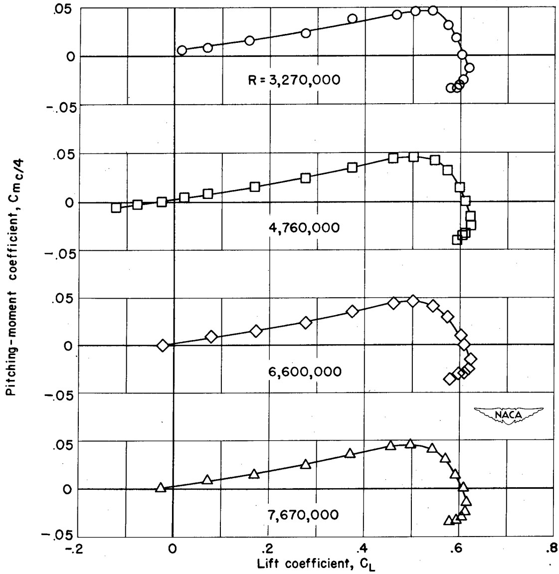
(b) Variation of C_{m_c/4} with C_L .
