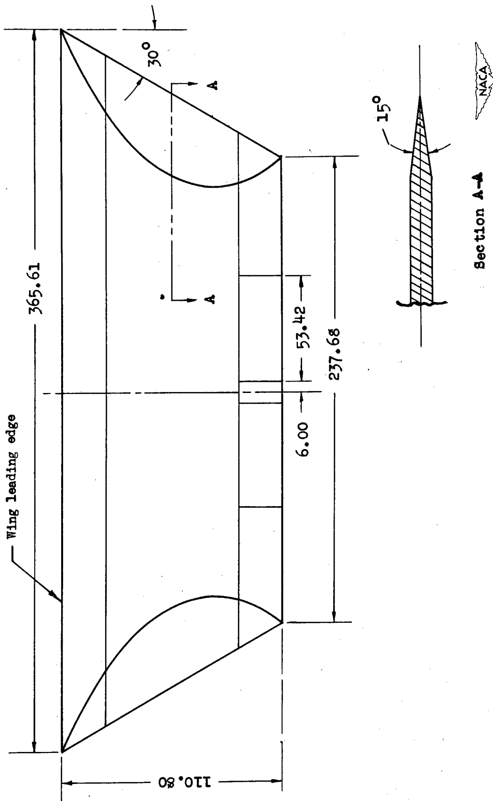
Figure 1.- Geometric characteristics of trapezoidal wing. Wing area, 232.0 square feet; aspect ratio, 4.0. All dimensions are given in inches.
